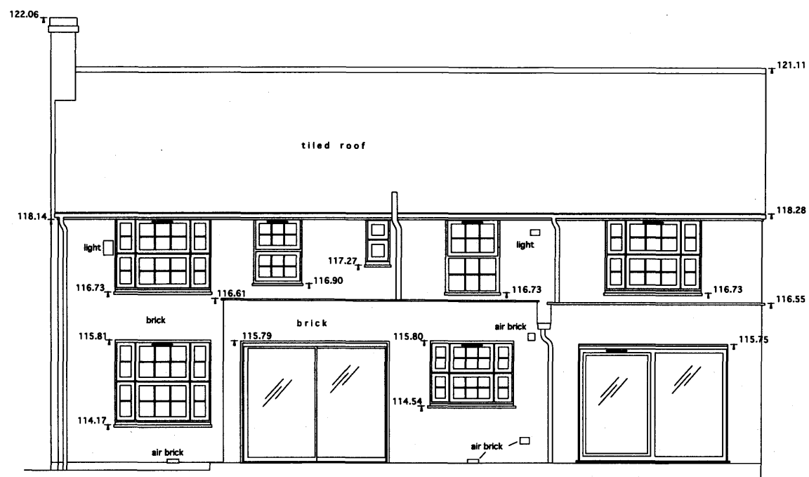
South Elevation
