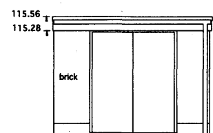
Garage South Elevation
