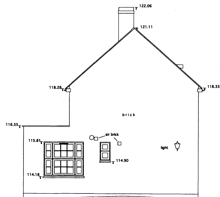
West Elevation
