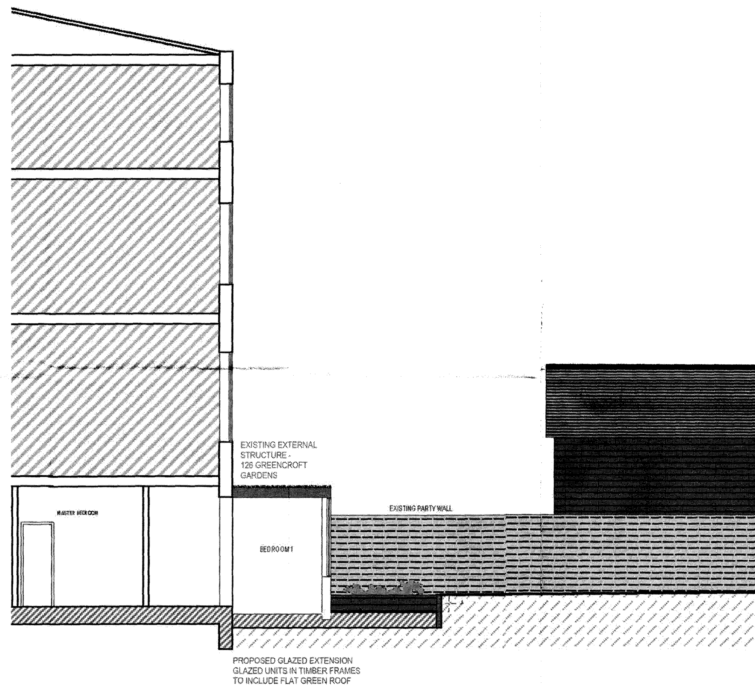
7 PROPOSED INTERNAL SECTION scale 1:50
