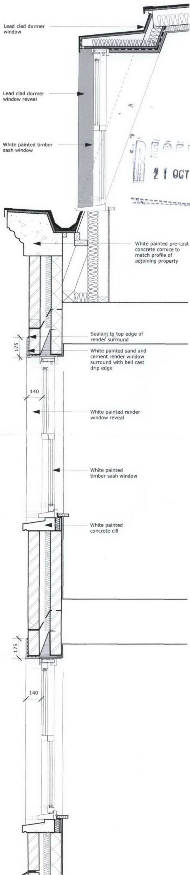
Section 1:20
