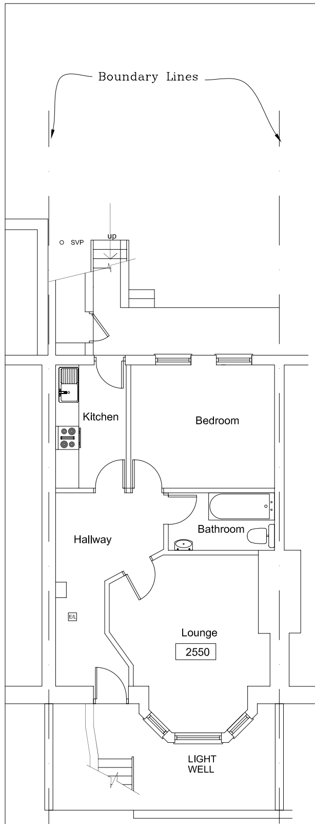
EXISTING LOWER GROUND FLOOR PLAN 1:100
