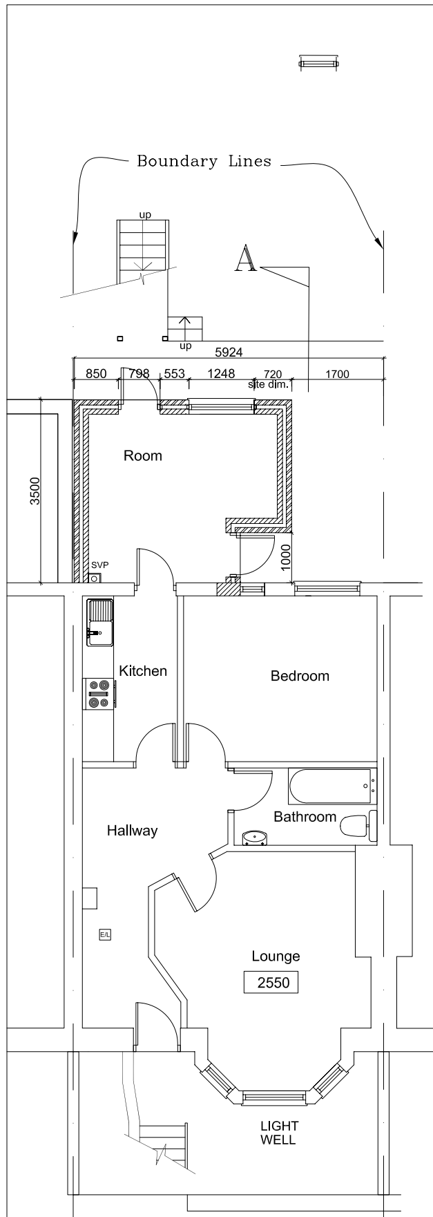
PROPOSED LOWER GROUND FLOOR PLAN 1:100
