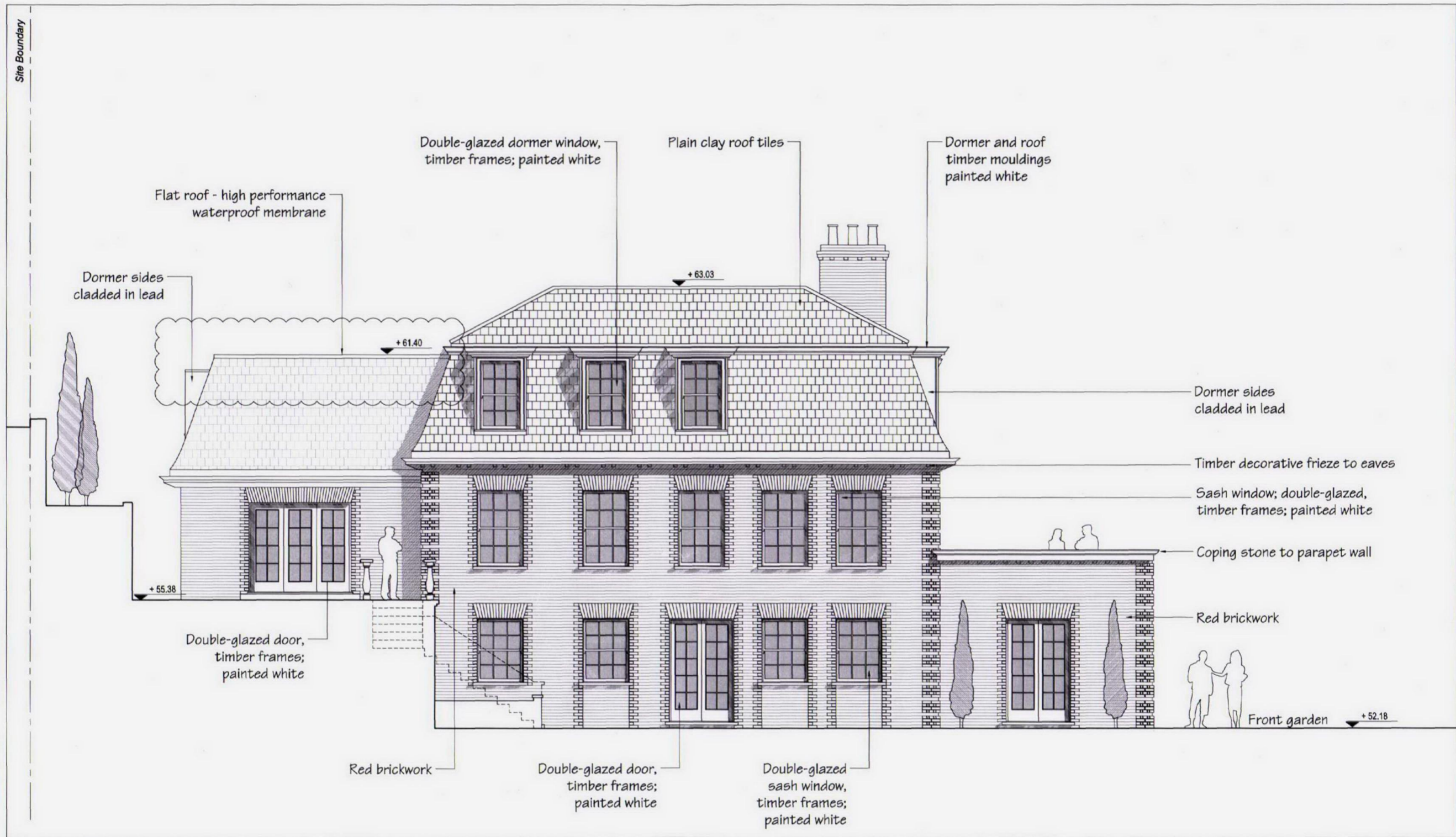
Proposed Side Elevation - North-West Scale 1:50 @A1
