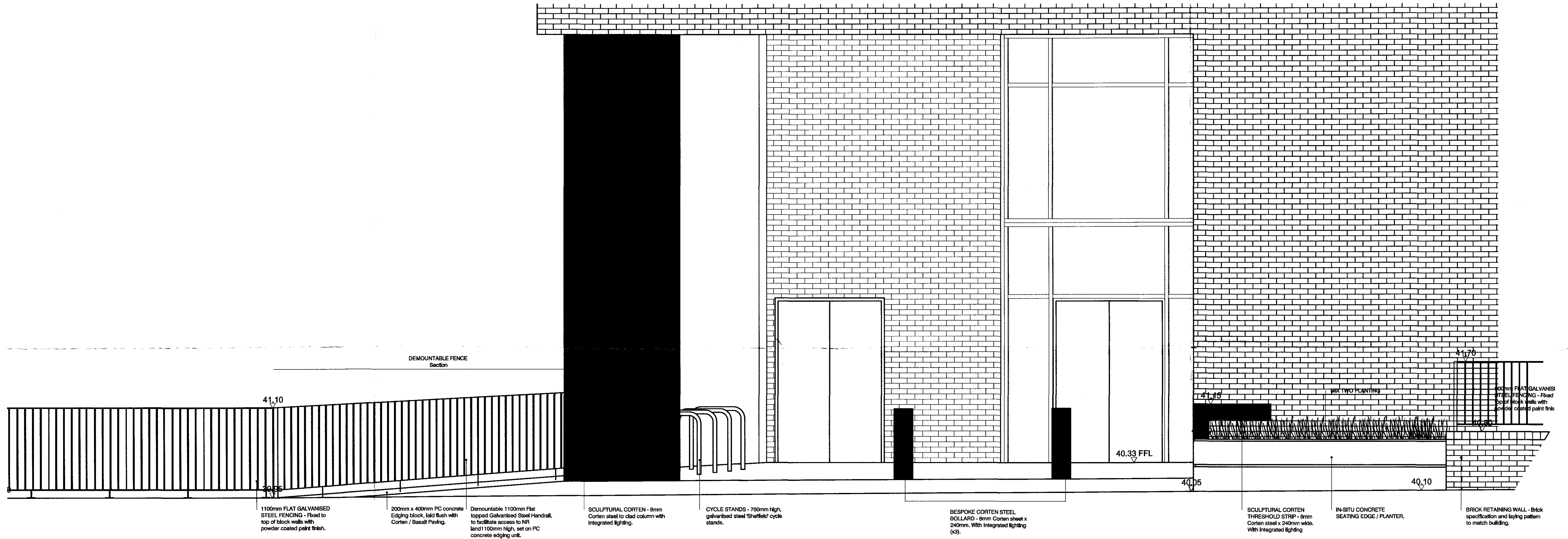
West Elevation Scale 1:25
