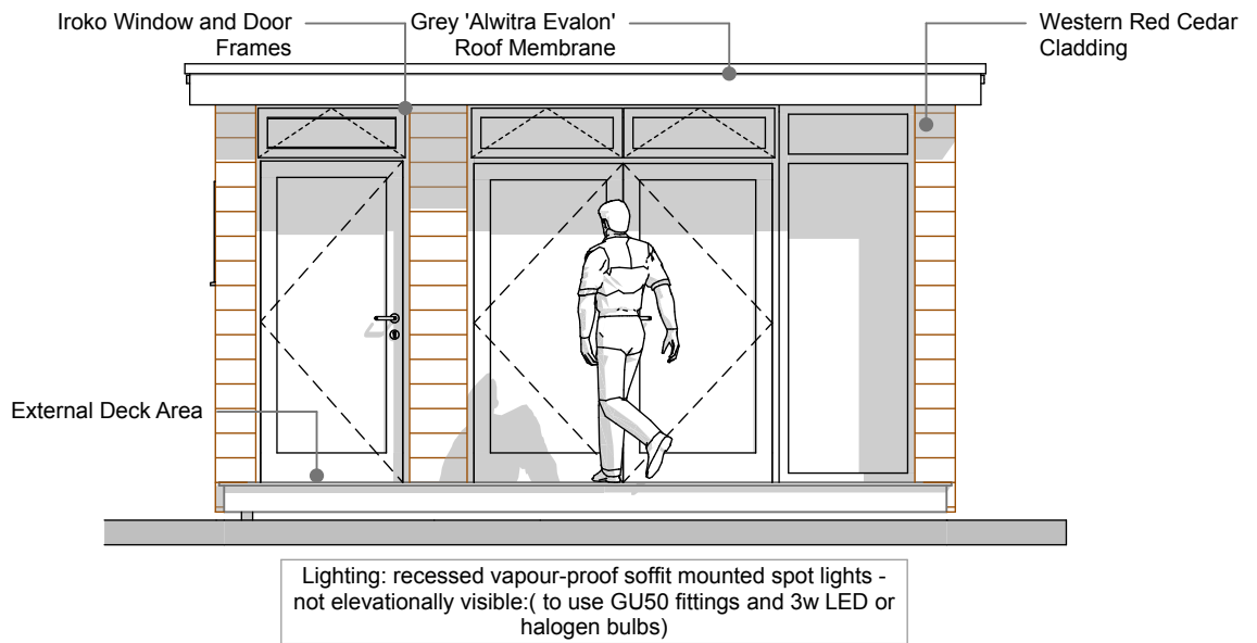
Front Elevation - 1:50
