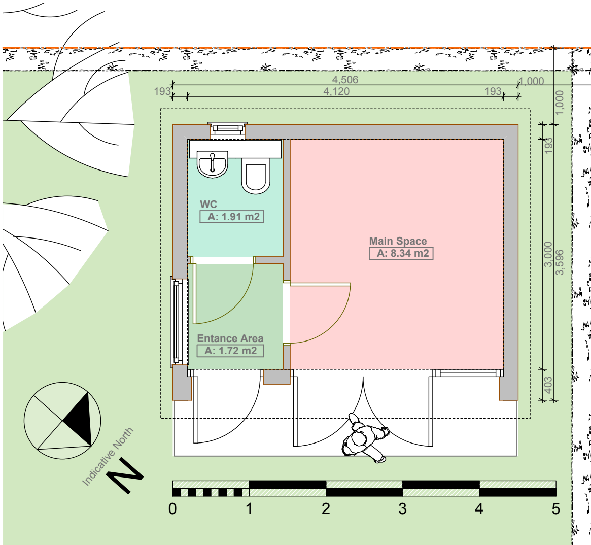
Floor Plan 1:50
