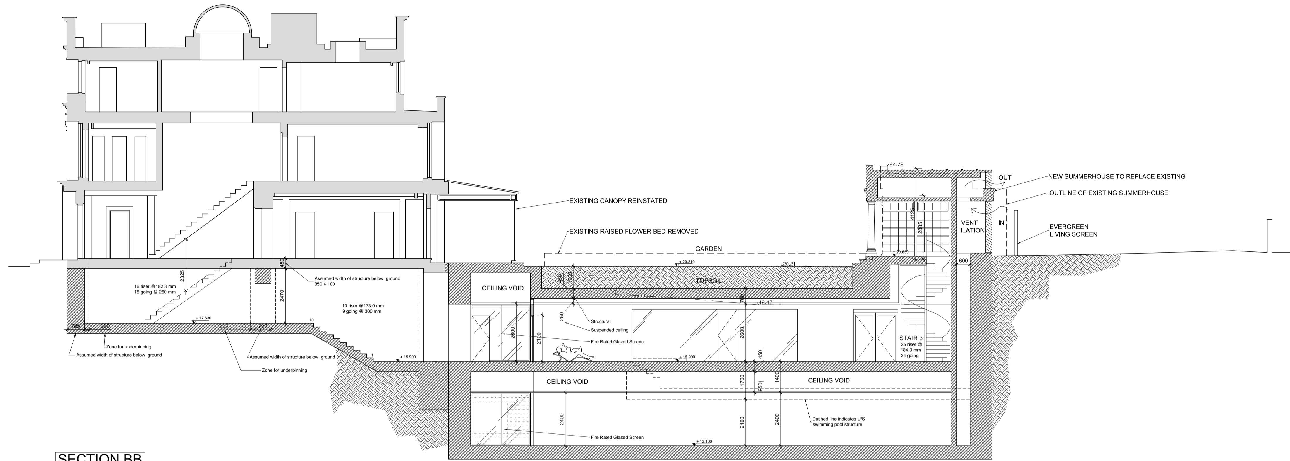
SECTION BB
