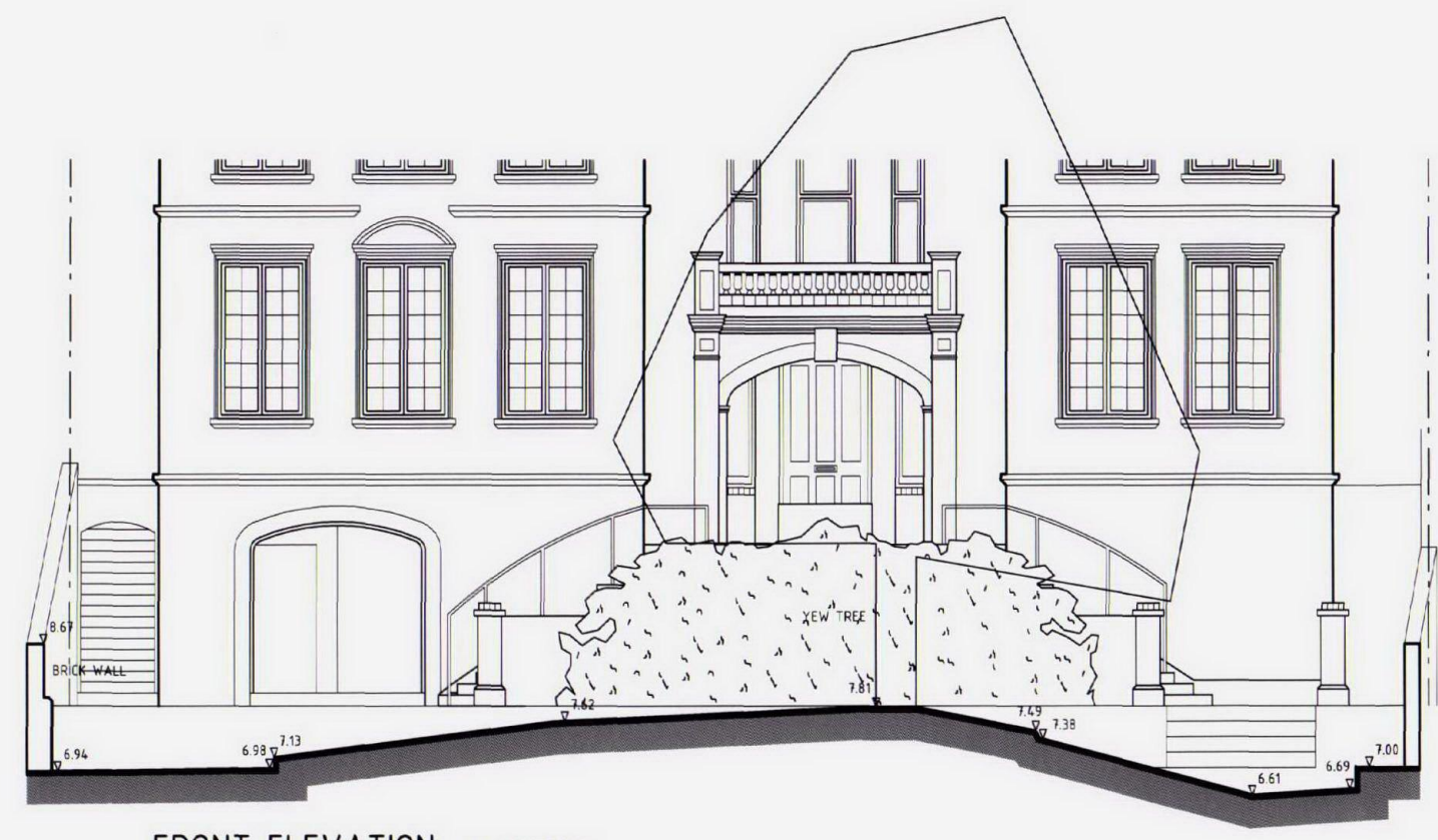
FRONT ELEVATION (AS EXISTING)
