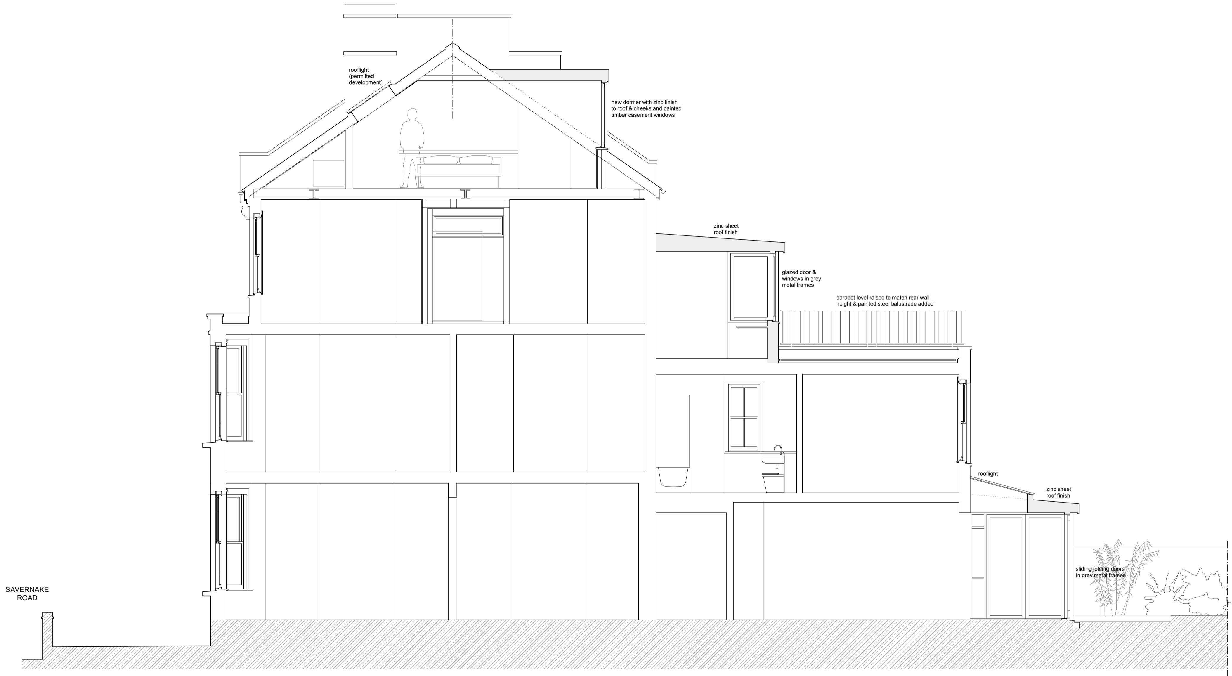
SECTION B - B LOOKING WEST
