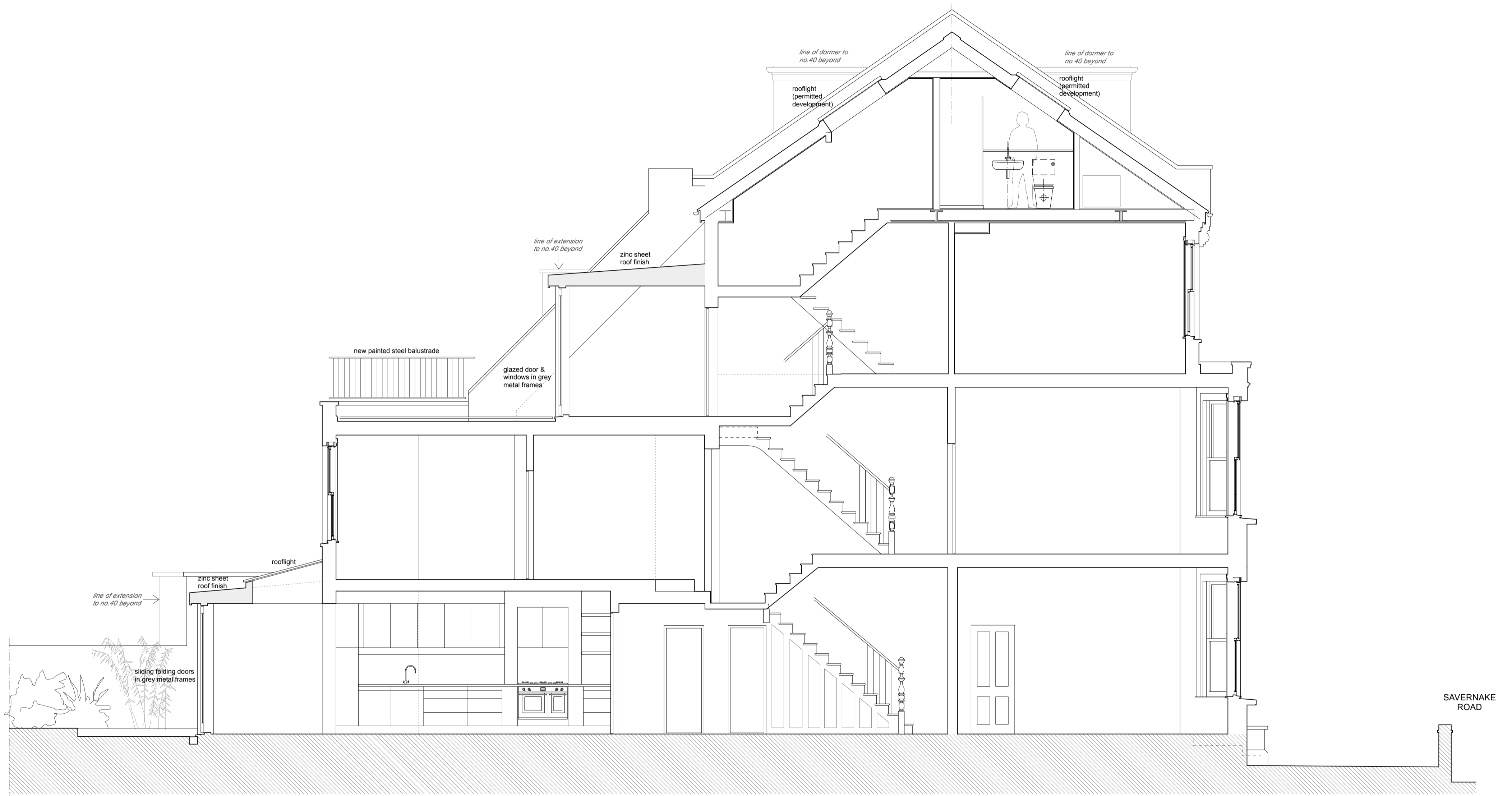
SECTION A - A LOOKING EAST
