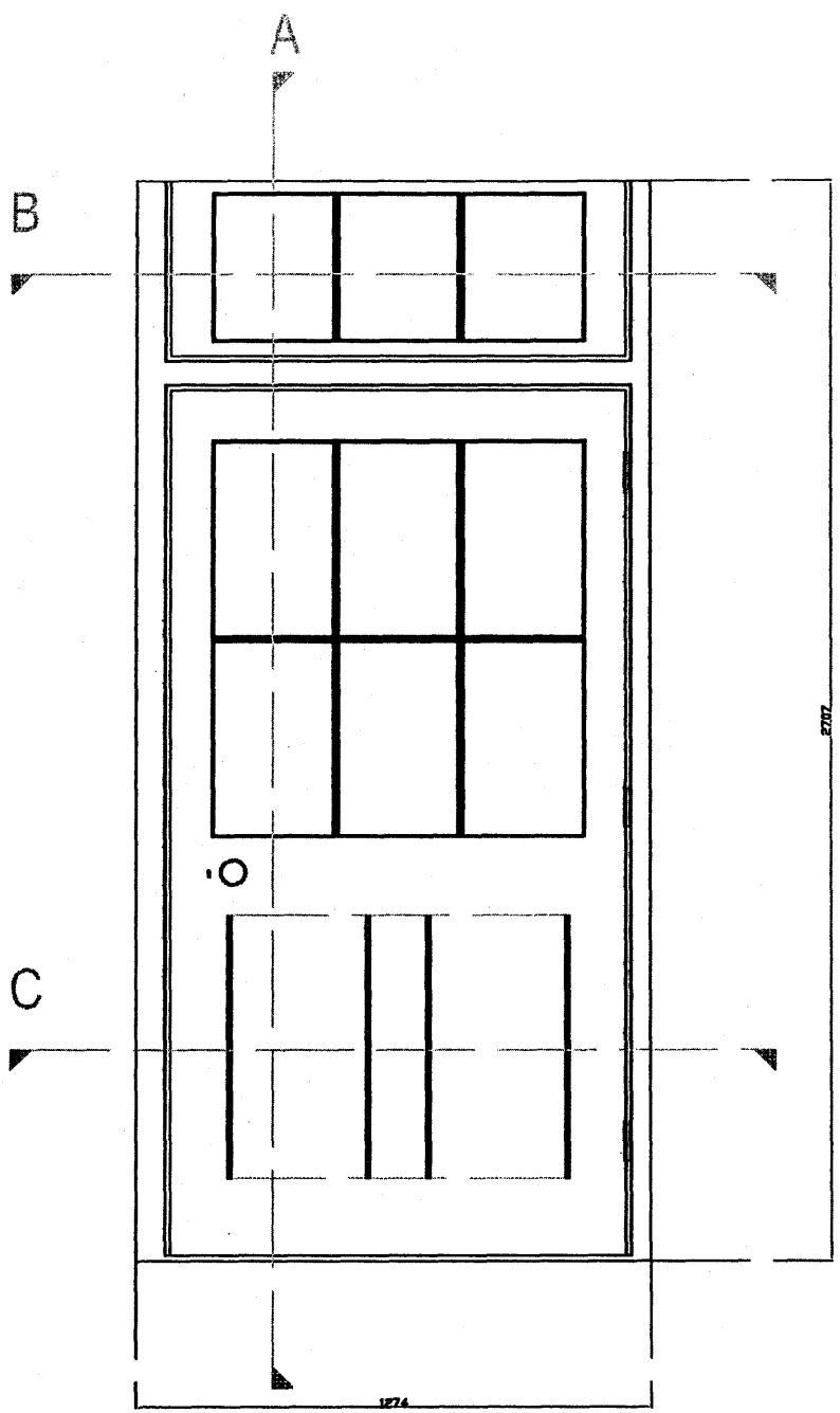
Internal Elevation
