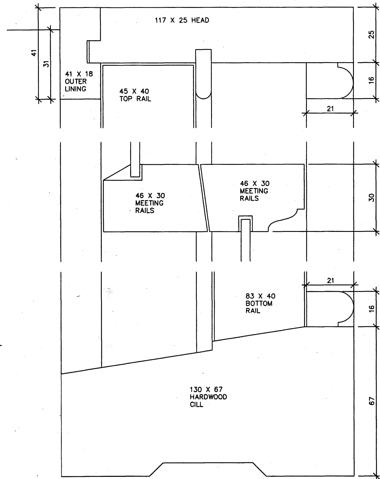
WIDTH SECTION SCALE FULL SIZE
