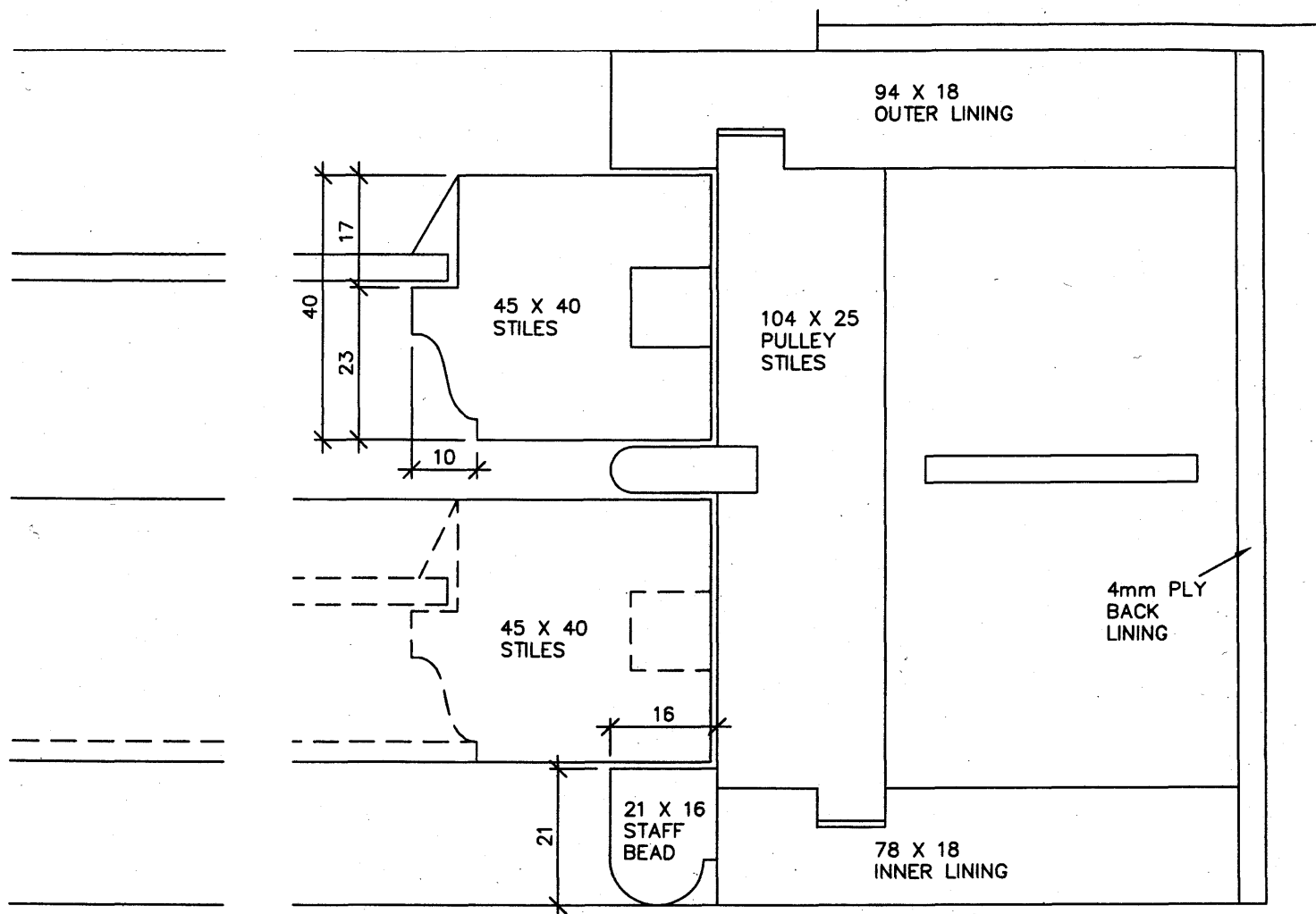
WIDTH SECTION SCALE FULL SIZE
