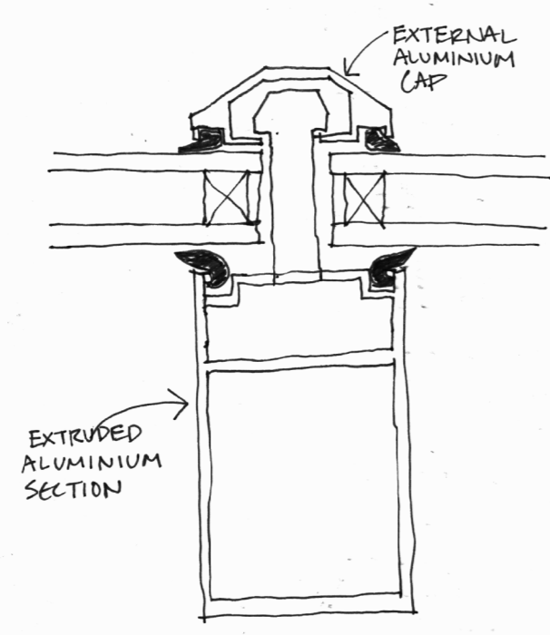
01 EXISTING ROOF GLAZING SECTION 289 SCALE 1:1
