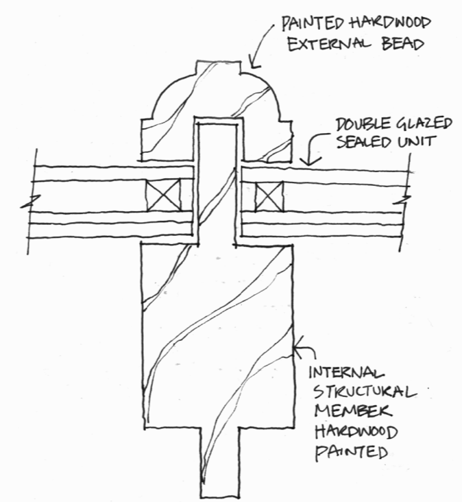
01 PROPOSED SECTION A-A 289 SCALE 1:1
