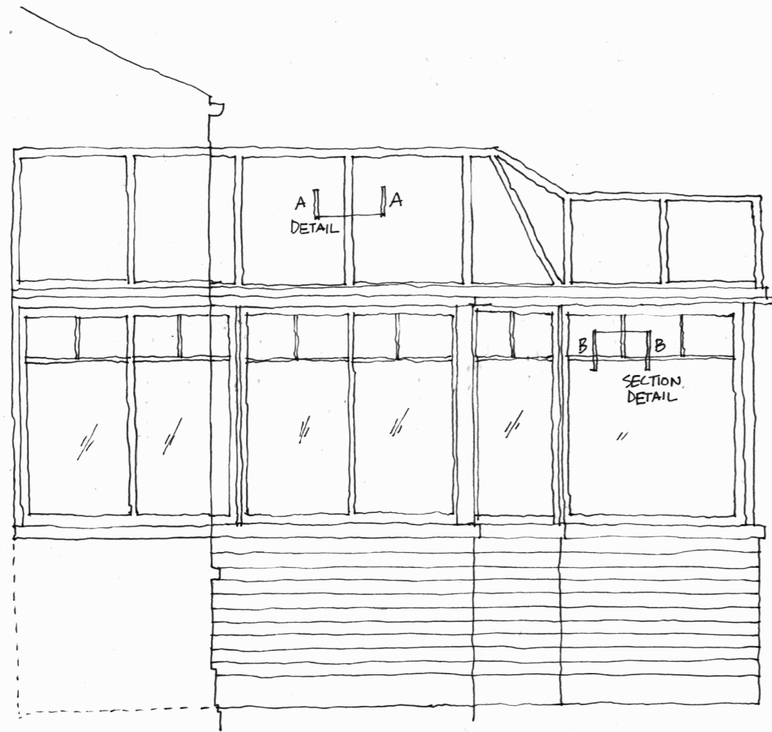
01 PROPOSED ELEVATION 289 SCALE 1:20
