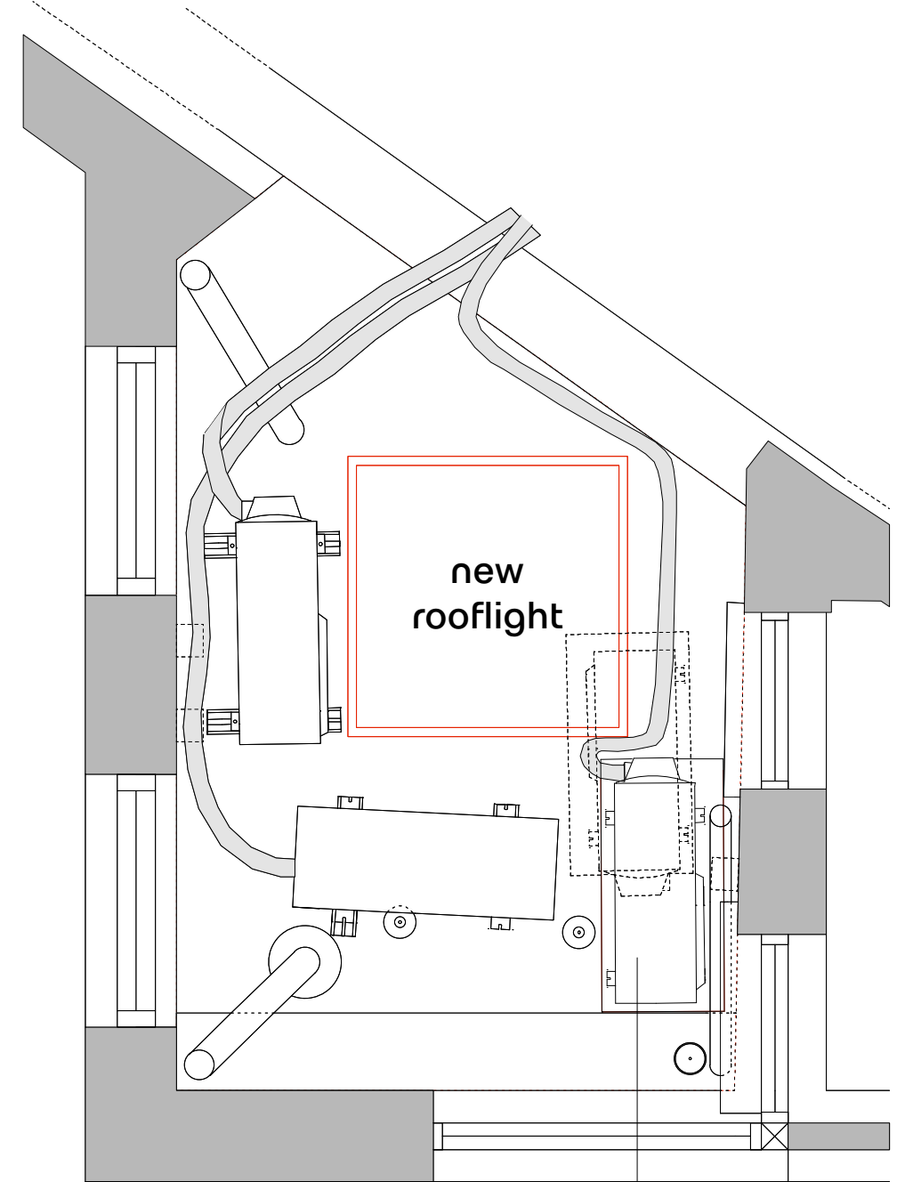
proposed roof
