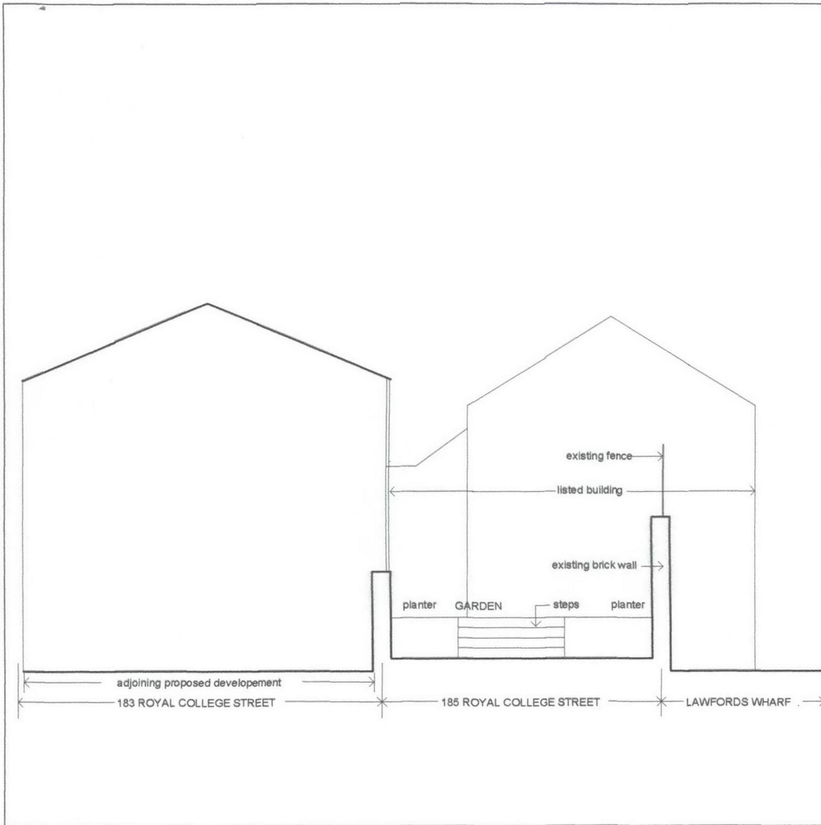
PROPOSED SECTION 4
