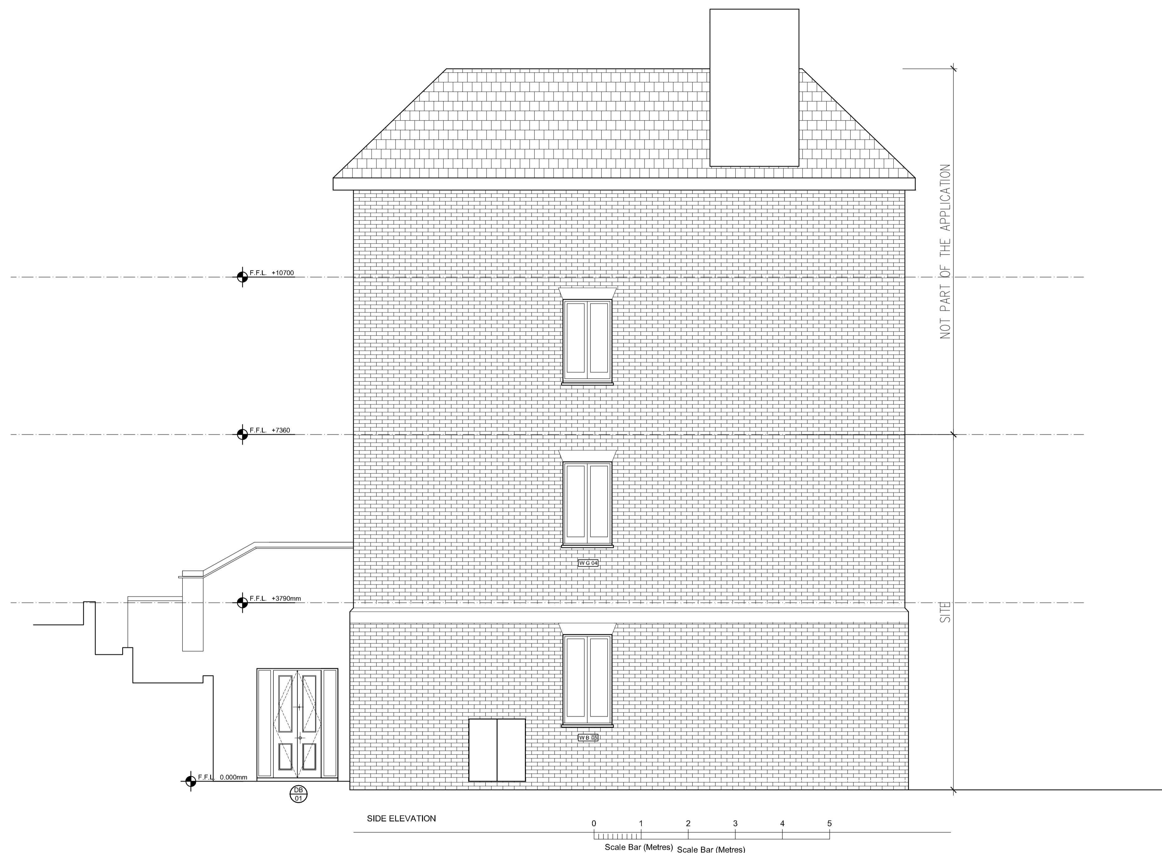
SIDE ELEVATION
