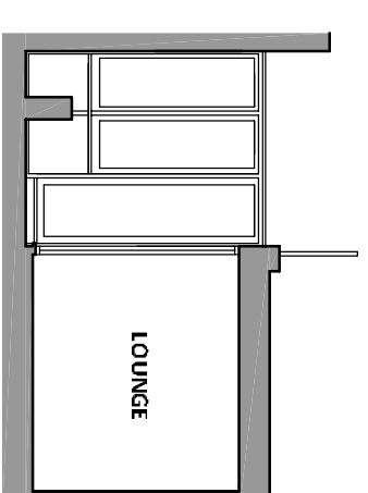
Proposed Section B-B
