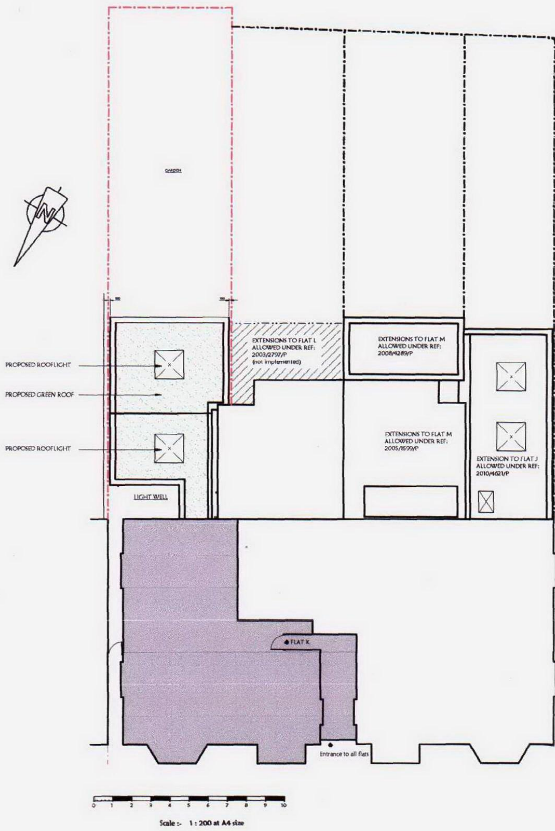
BLOCK / ROOF PLAN for FLAT K, 37 ARKWRIGHT ROAD, LONDON, NW3 SCALE :- 1:200
