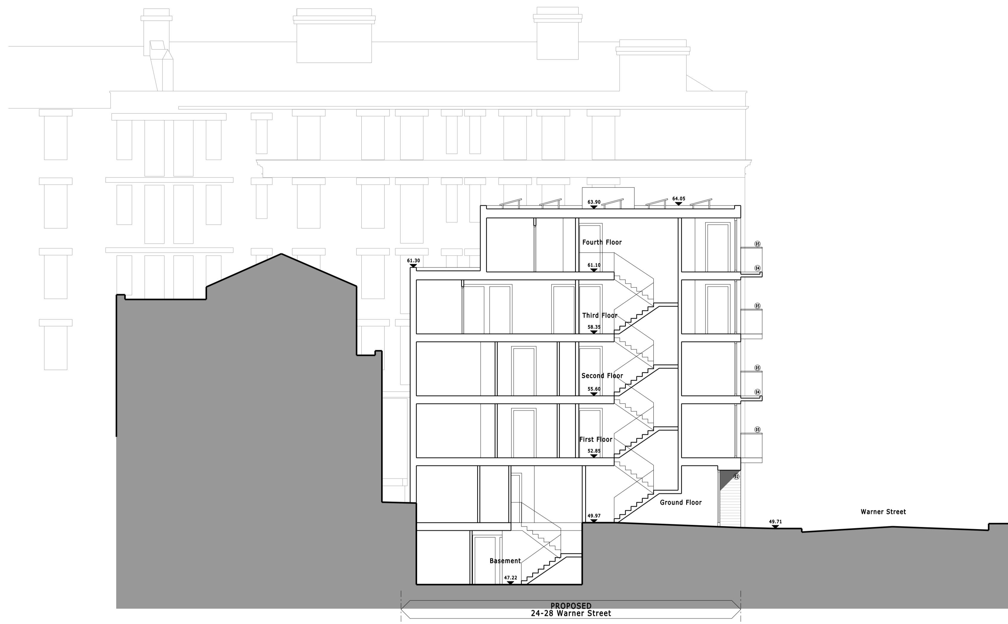
SECTION G-G
