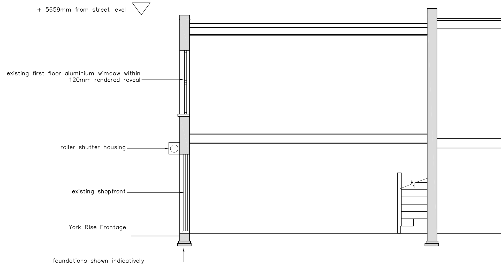
Existing Section A-A
