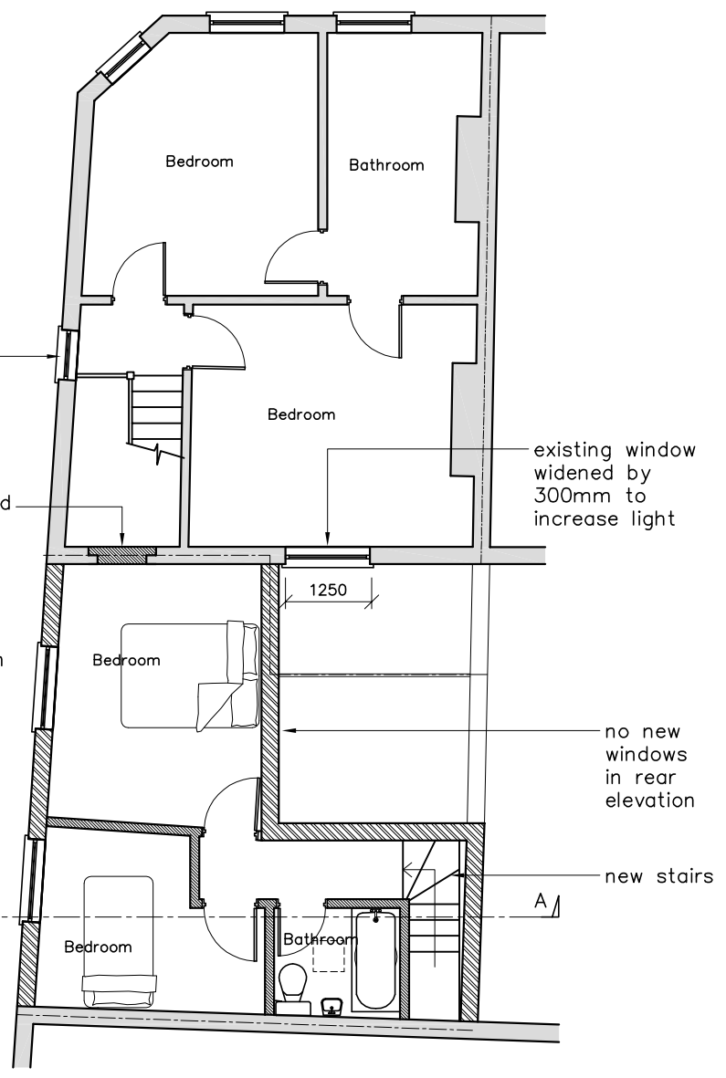
Proposed Second Floor Extension
