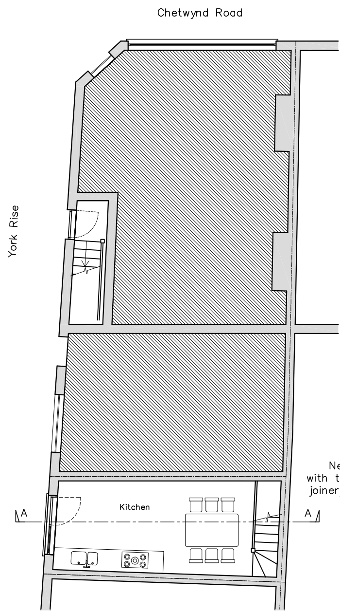
Proposed Ground Floor Reconfiguration
