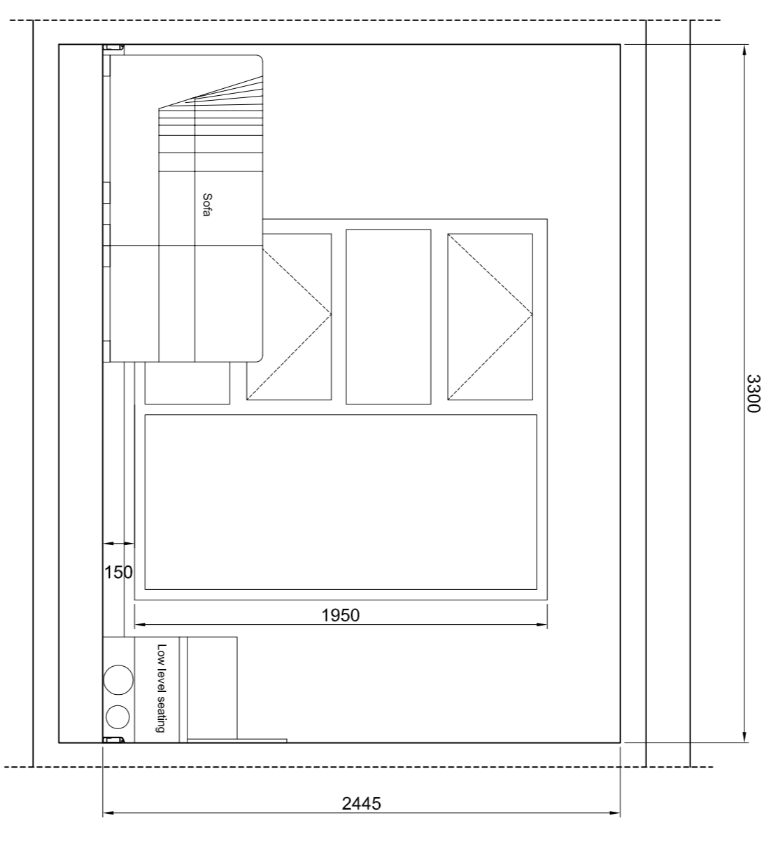
ELEVATION D
