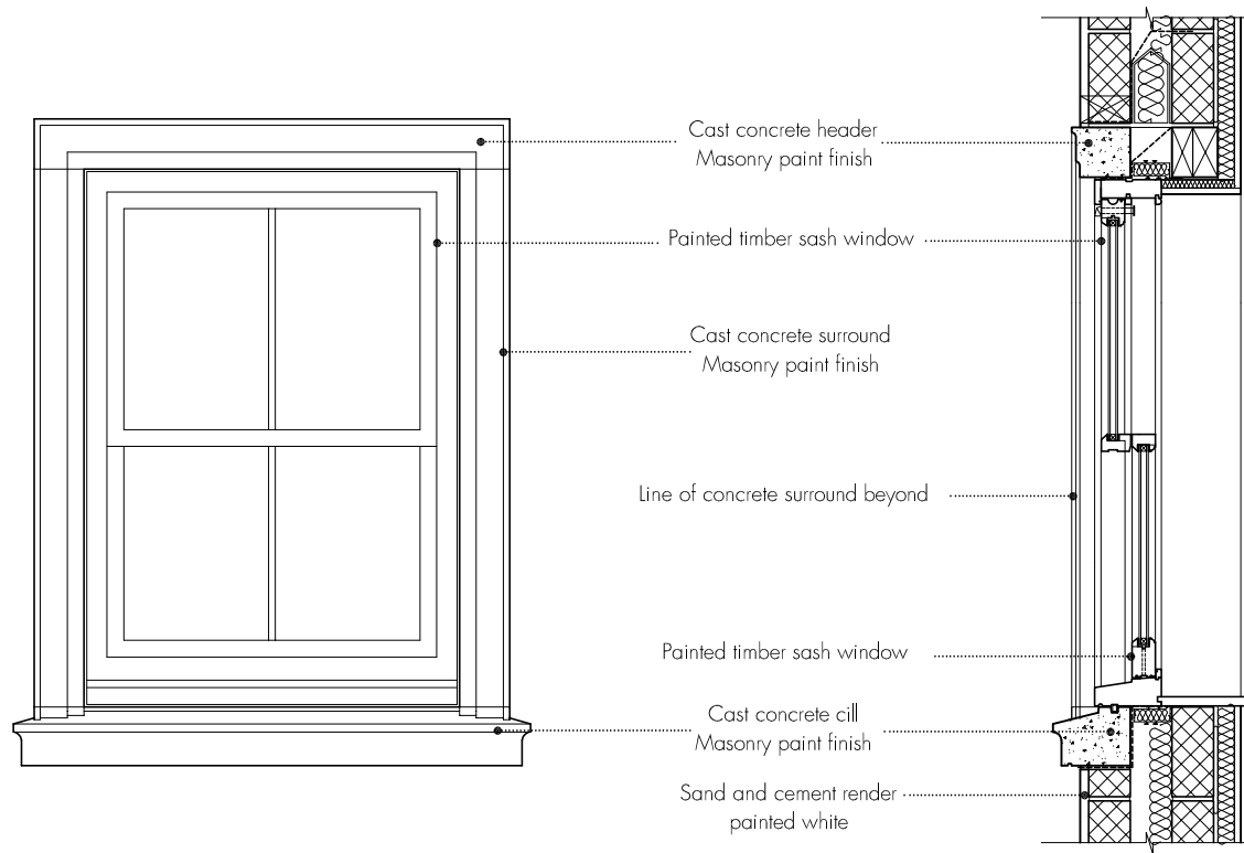
TYPICAL WINDOW/ SURROUND ELEVATION 1:20
