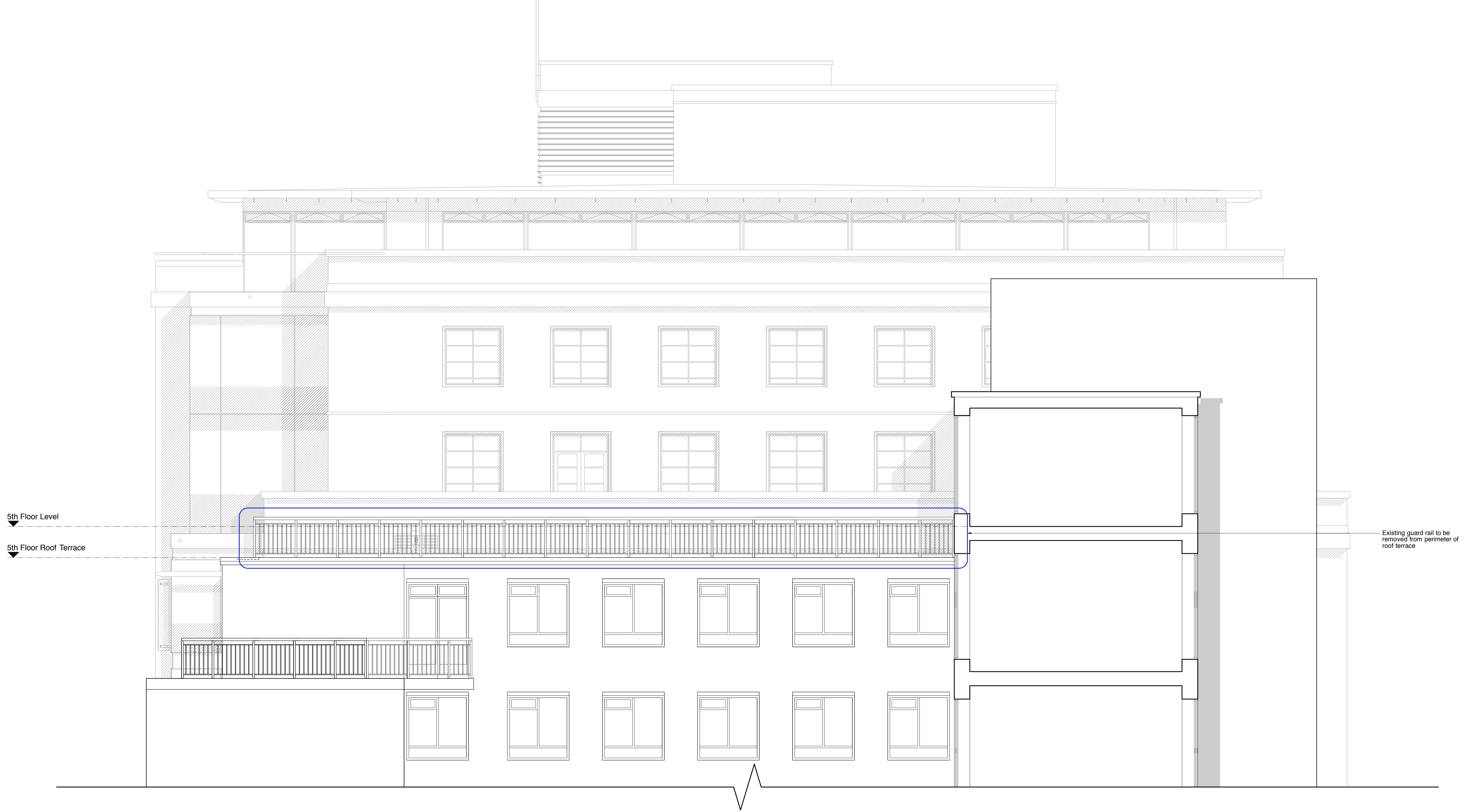
1 Existing North Elevation 2002 Scale: 1:50
