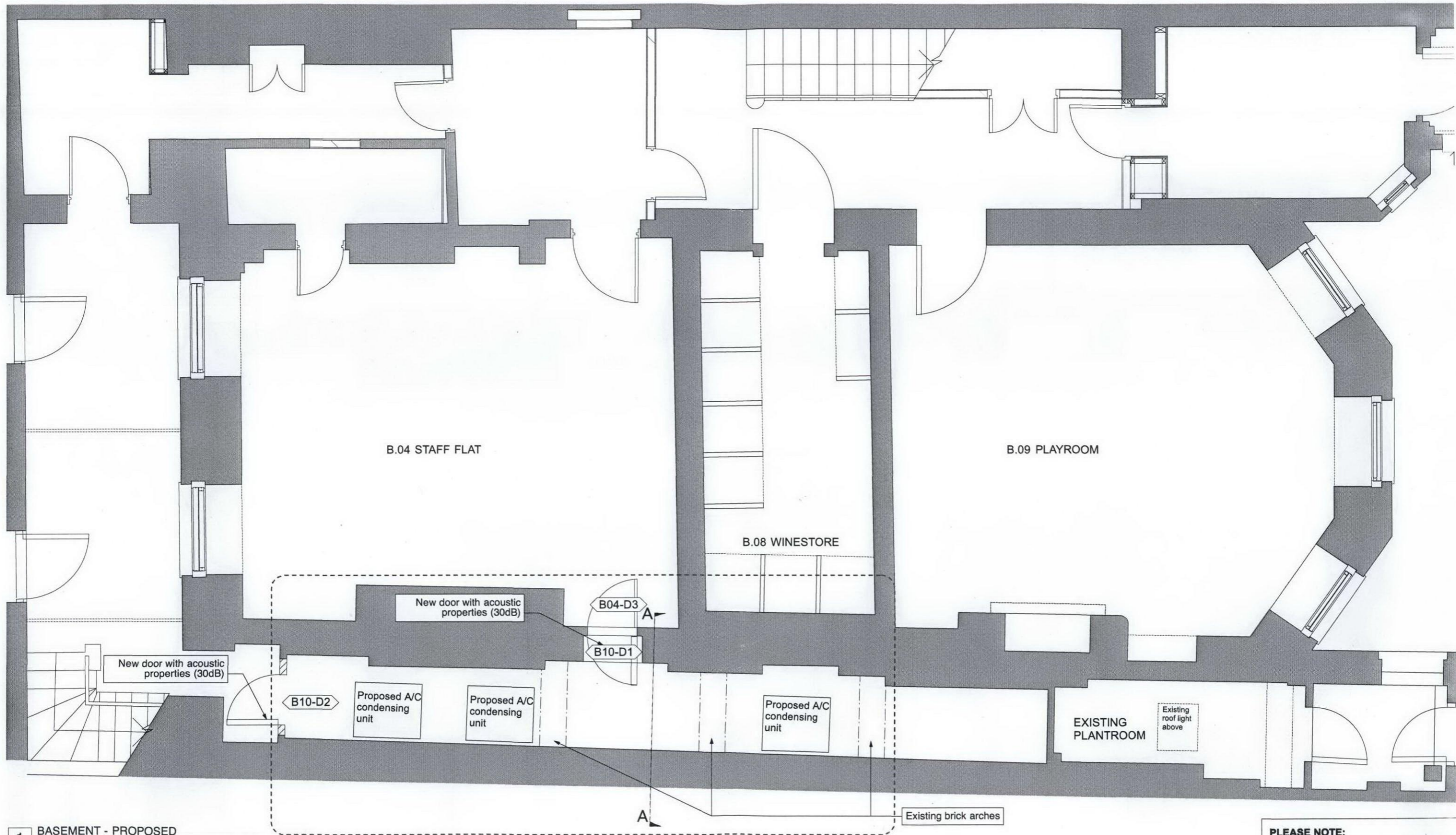
1 BASEMENT - PROPOSED SCALE 1:50
