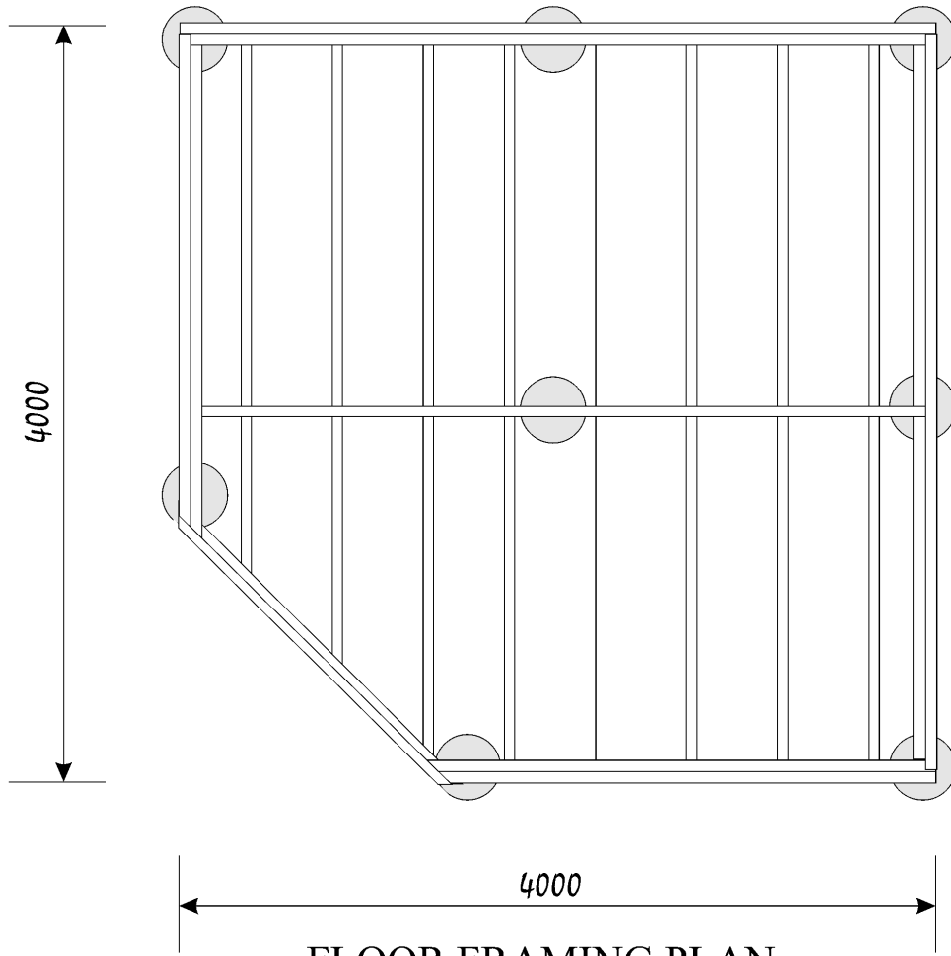
FLOOR FRAMING PLAN
