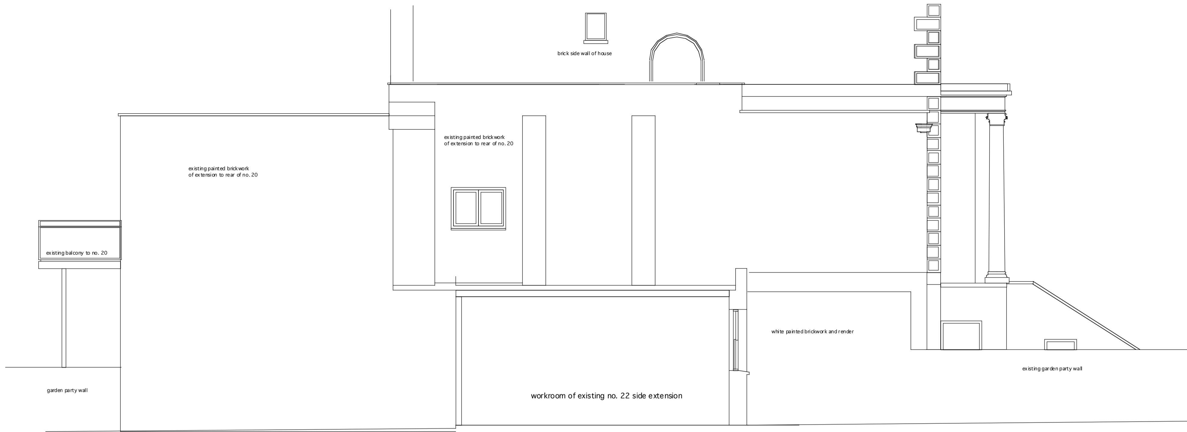
Existing Section CC through extension looking towards side wall of 20 UPR
