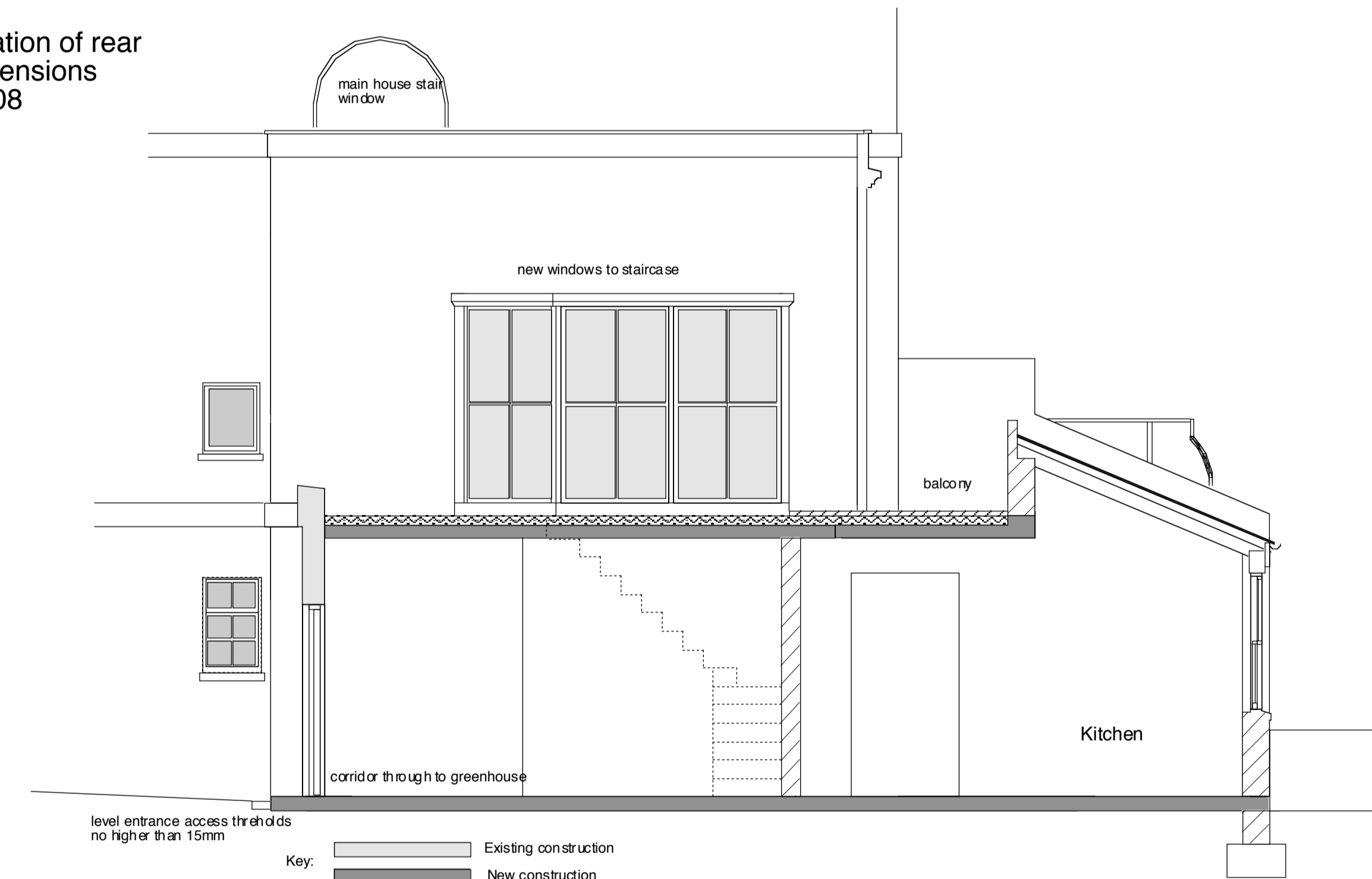
Proposed Section DD through enlarged extension looking towards side wall of 22 UPR
