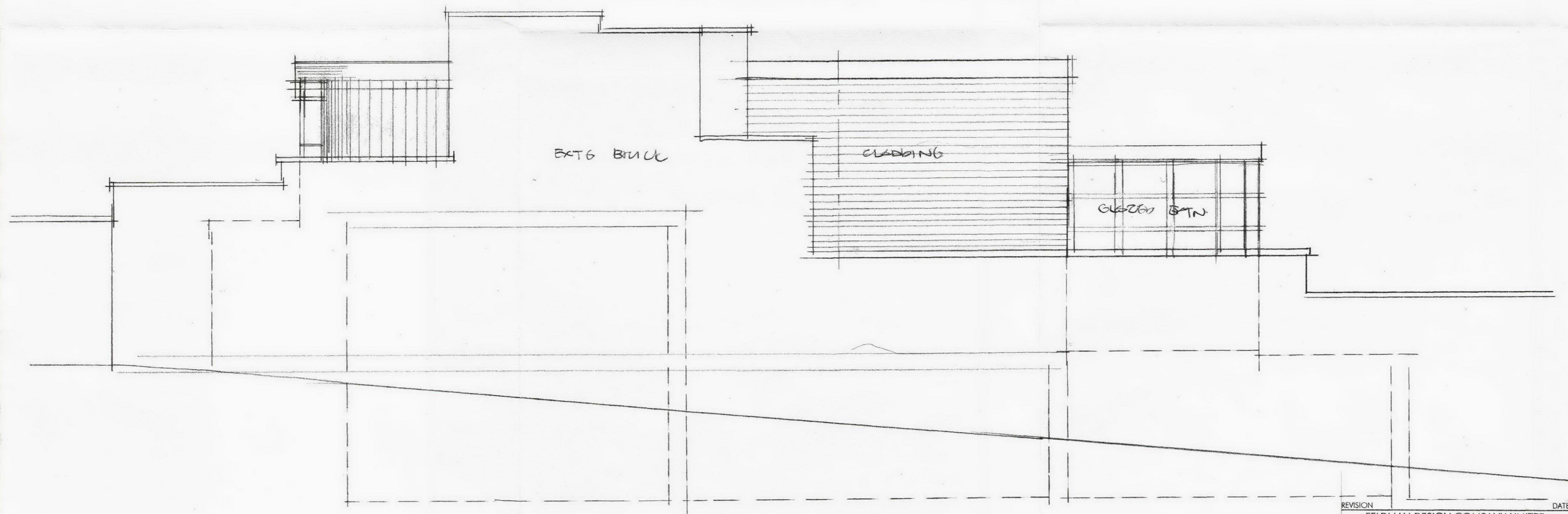
WEST ELEVATION (HEATH)
