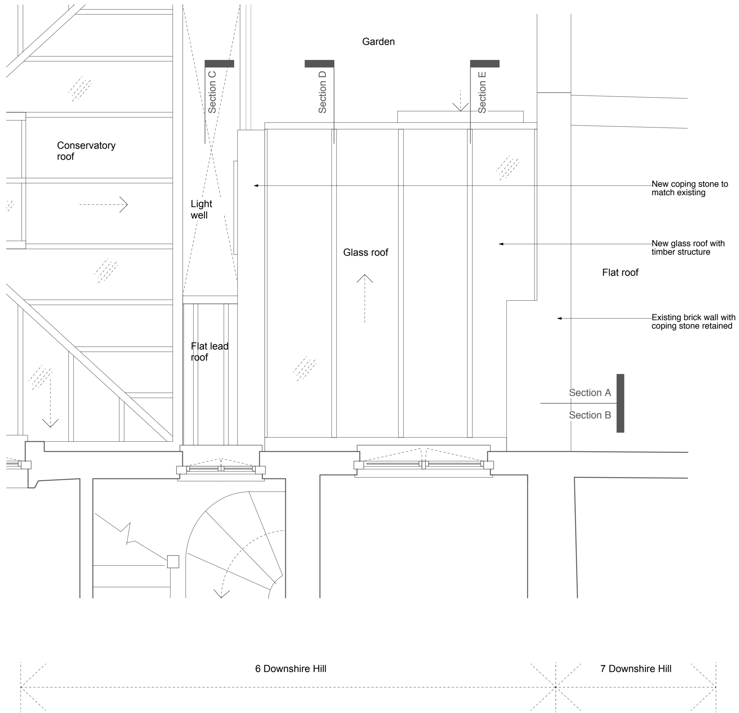
Garden Entry Detail Proposal - First Floor Plan (roof over garden entrance hall)
