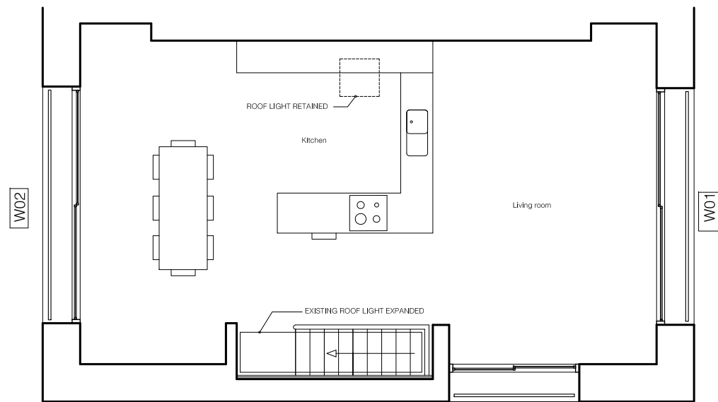
01 PROPOSED THIRD FLOOR PLAN 1.100 PL03
