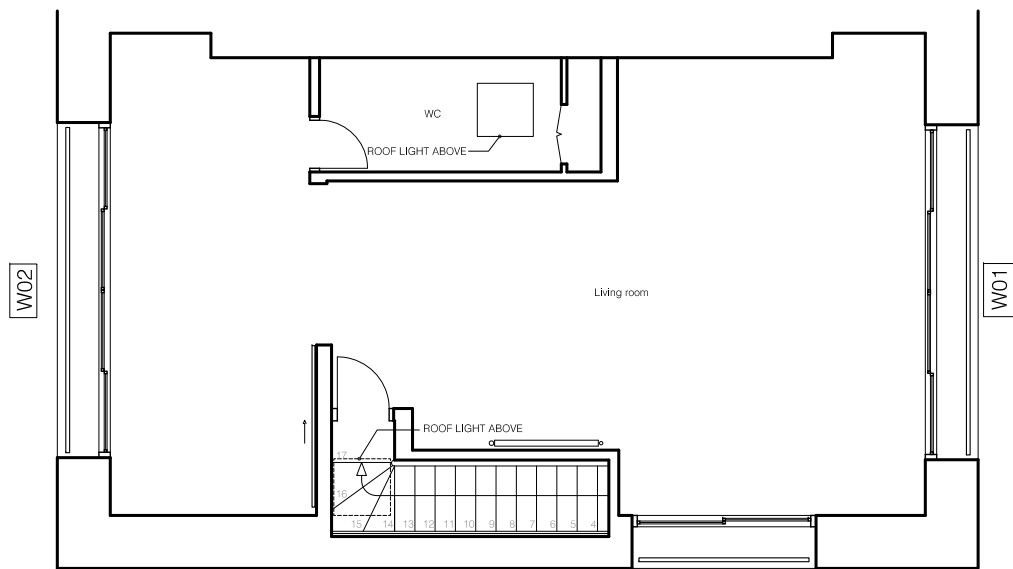
01 EXISTING THIRD FLOOR PLAN 1.100 PL03
