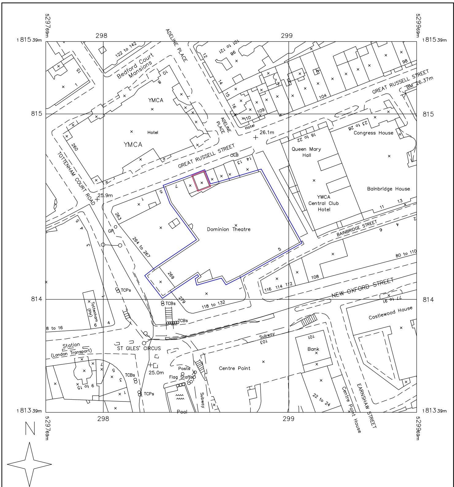
LOCATION PLAN (1:1250)
