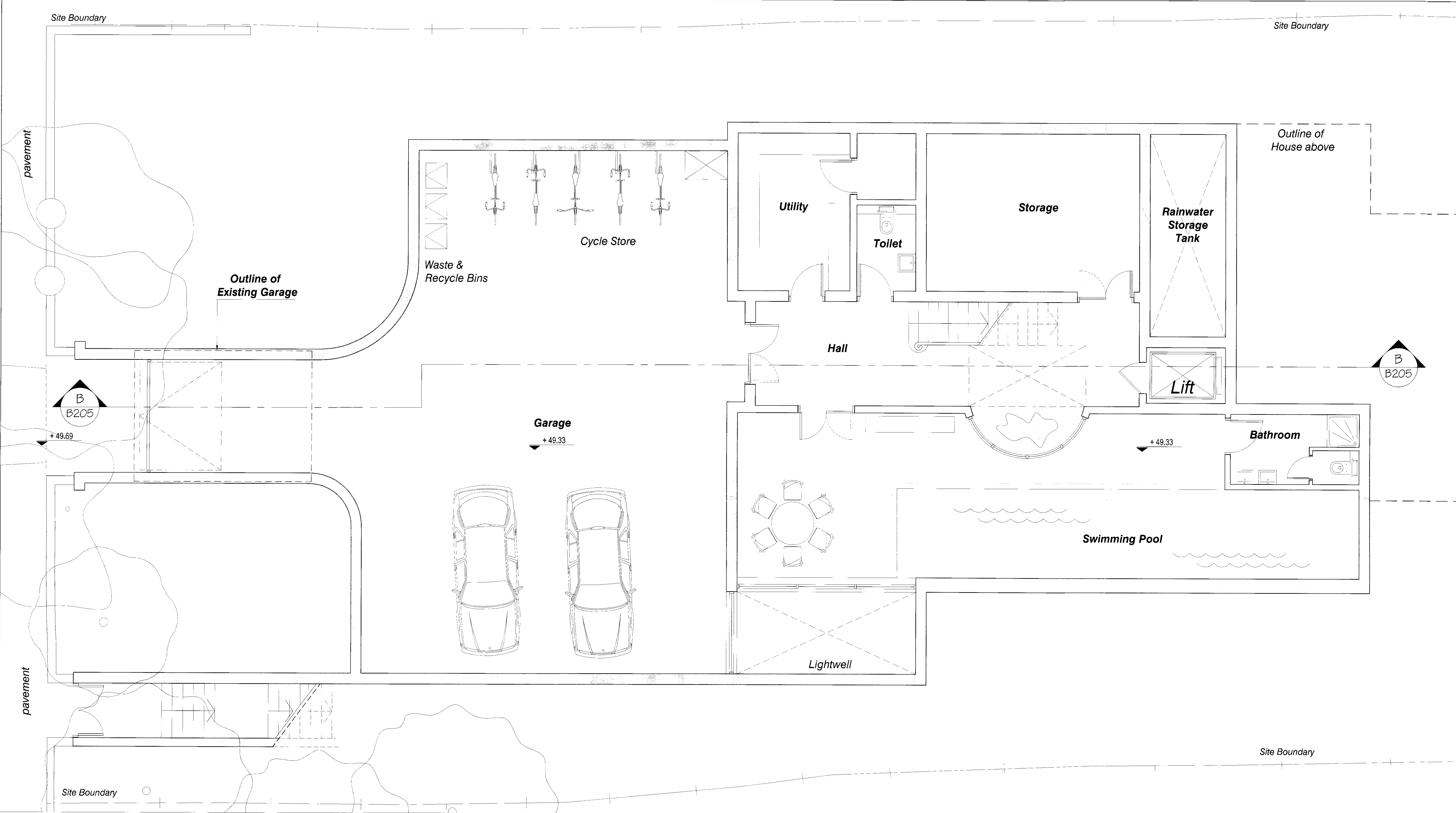
Proposed Garage Plan Scale 1:50 @A1
