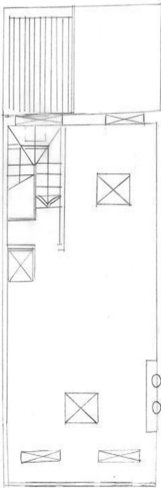
Drawing P4: Proposed roof alteration: floor plan for second floor
