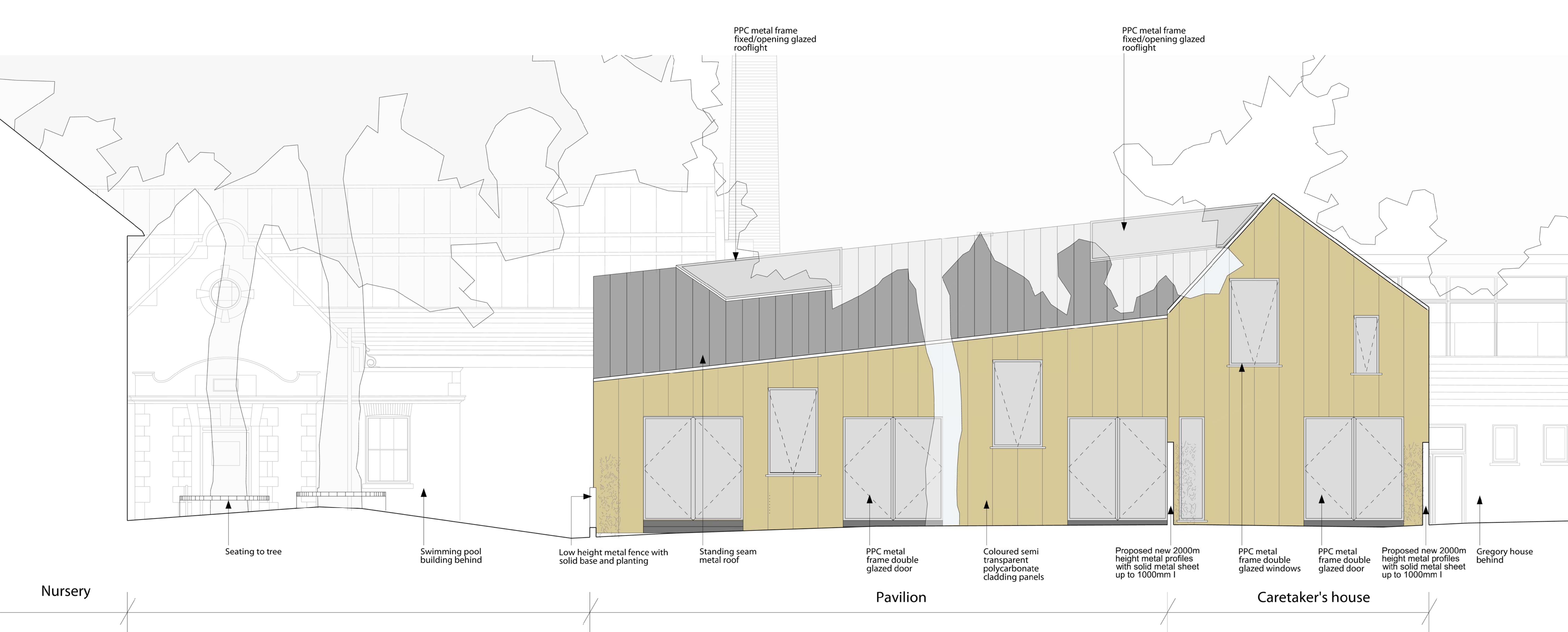
Proposed South Elevation
