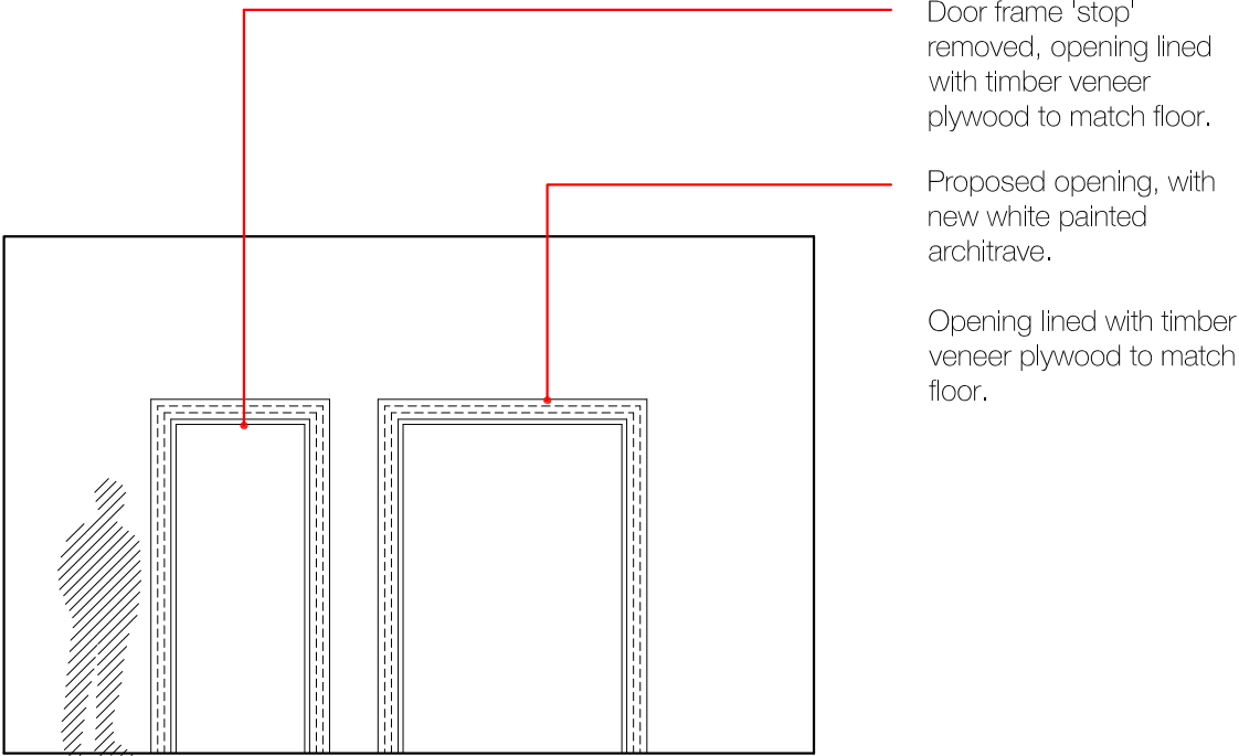
4. PROPOSED ELEVATION 1:20@A3
