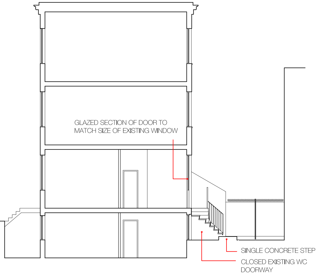
2. SECTION AA
