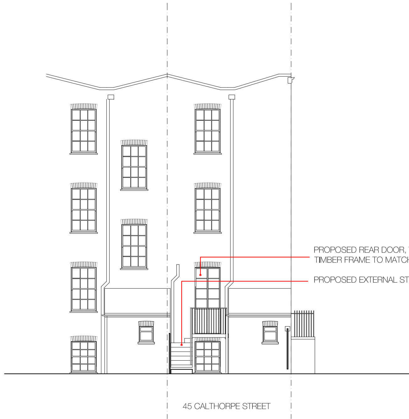
1. NORTH ELEVATION - REAR
