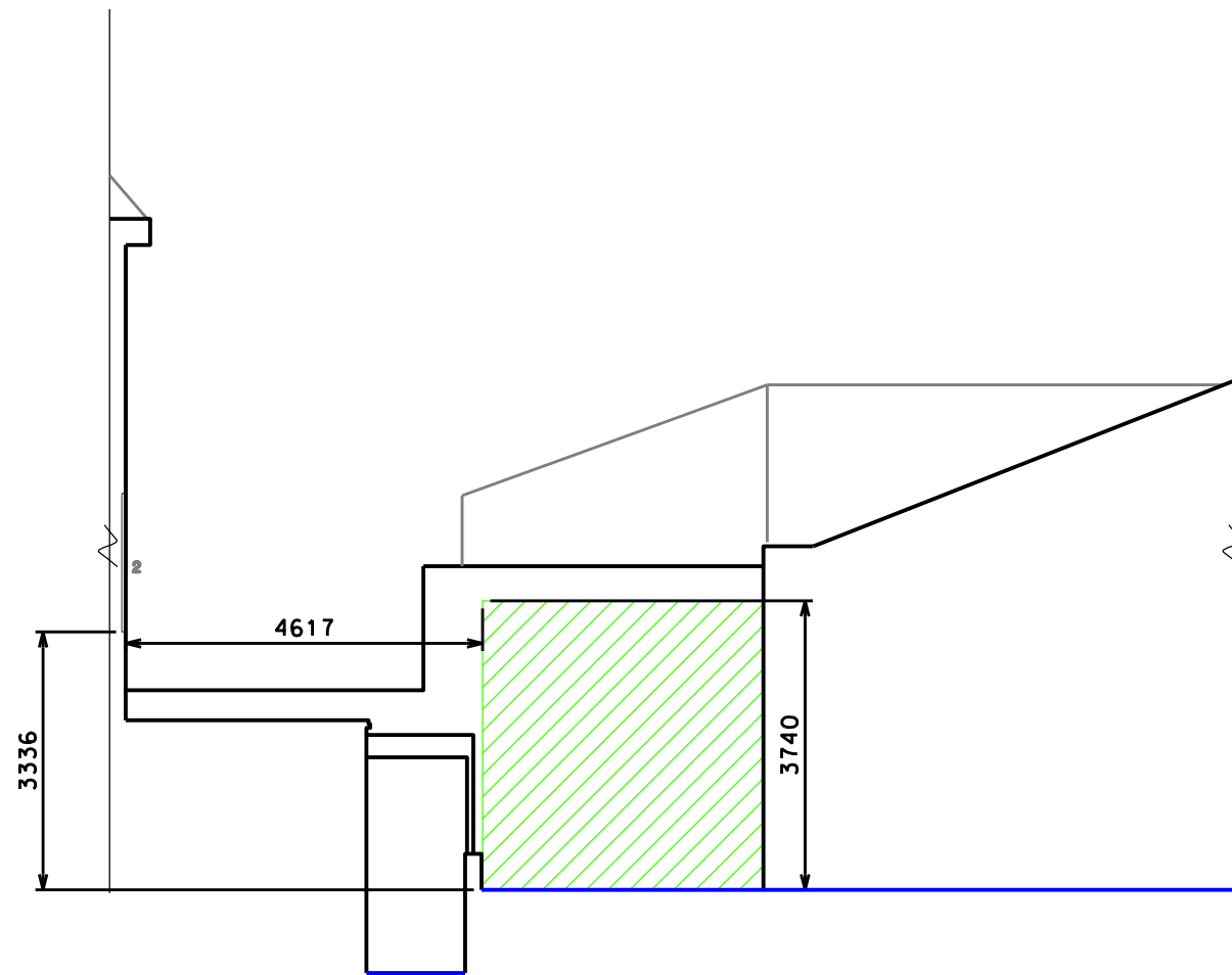
SECTION C-C
