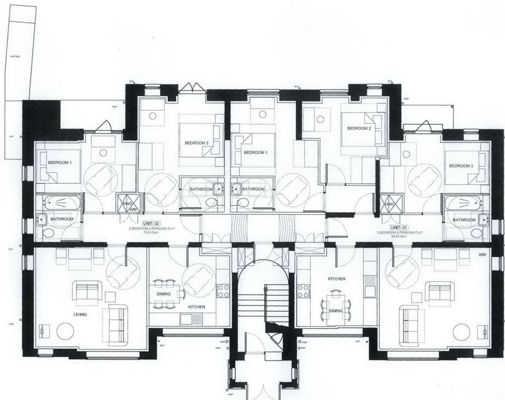
1 PROPOSED GROUND FLOOR PLAN 1:100
