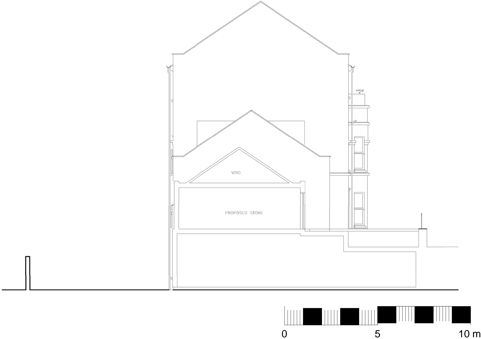
1 Proposed long section 1 : 100
