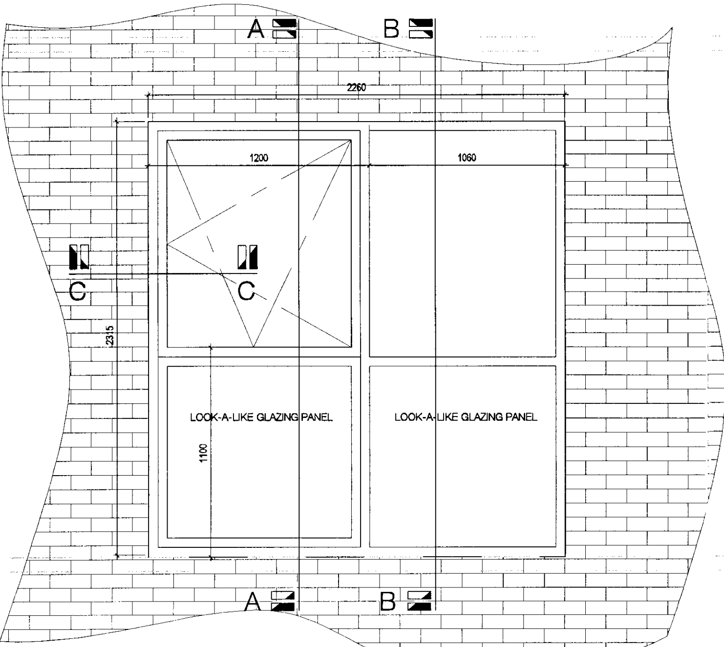
_ELEVATION SCALE 1:20
