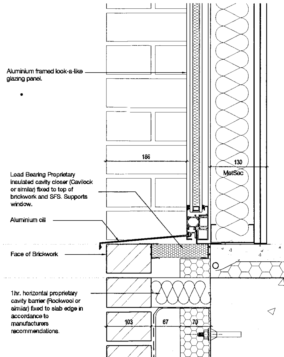
_CILL DETAIL_B SCALE 1:5
