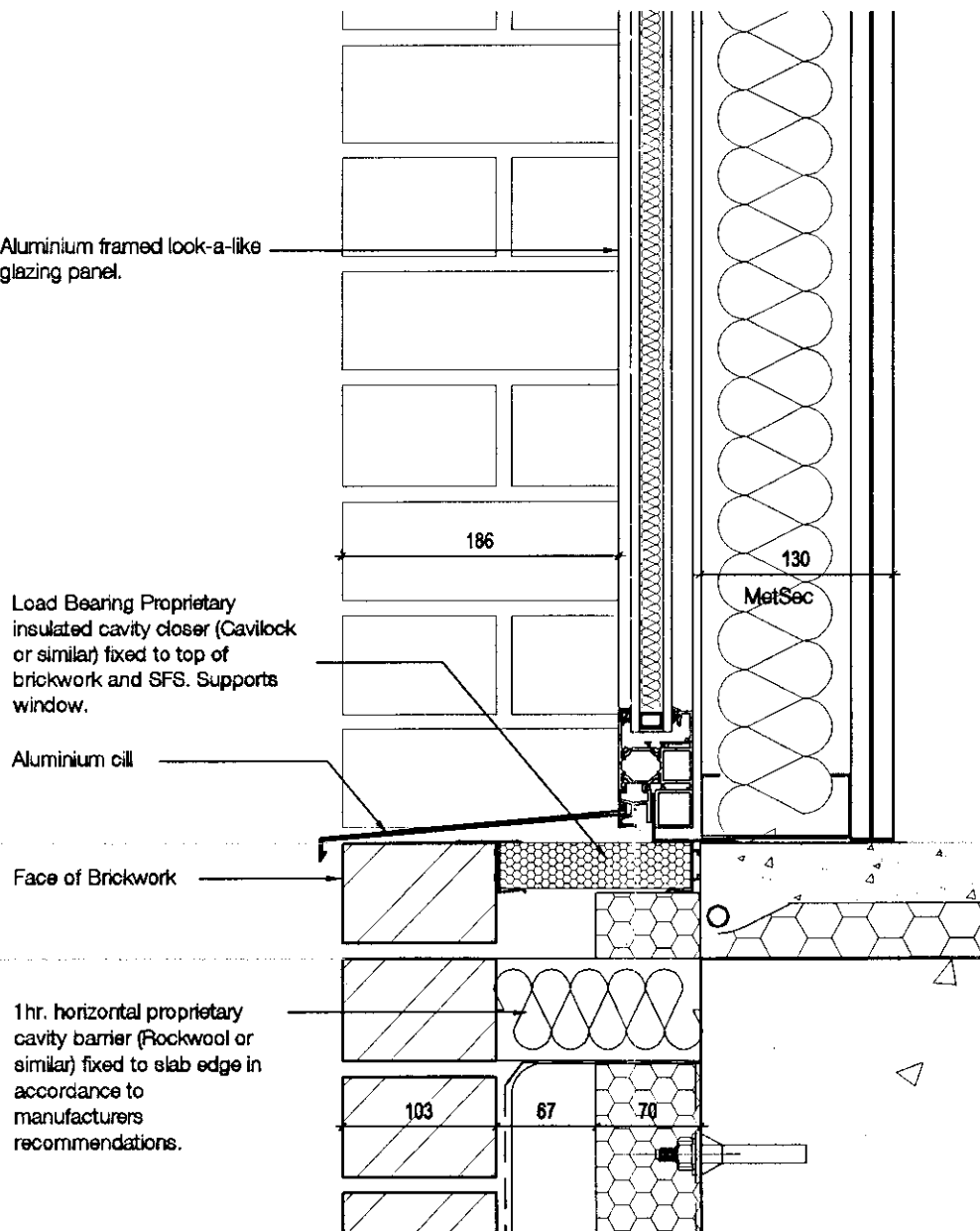
_CILL DETAIL_A SCALE 1:5
