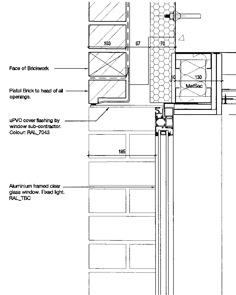
_HEAD DETAIL_B SCALE 1:5
