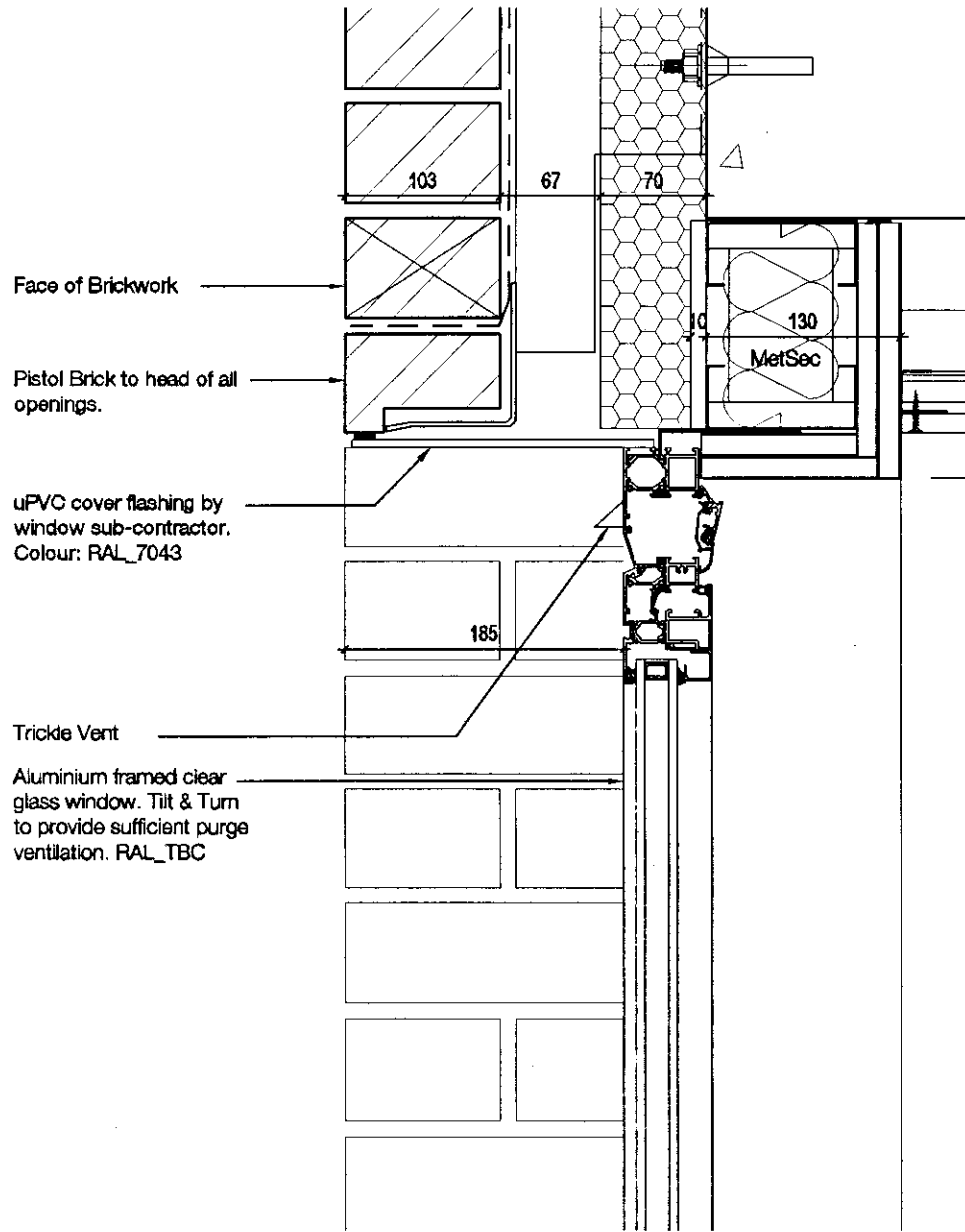
_HEAD DETAIL_A SCALE 1:5
