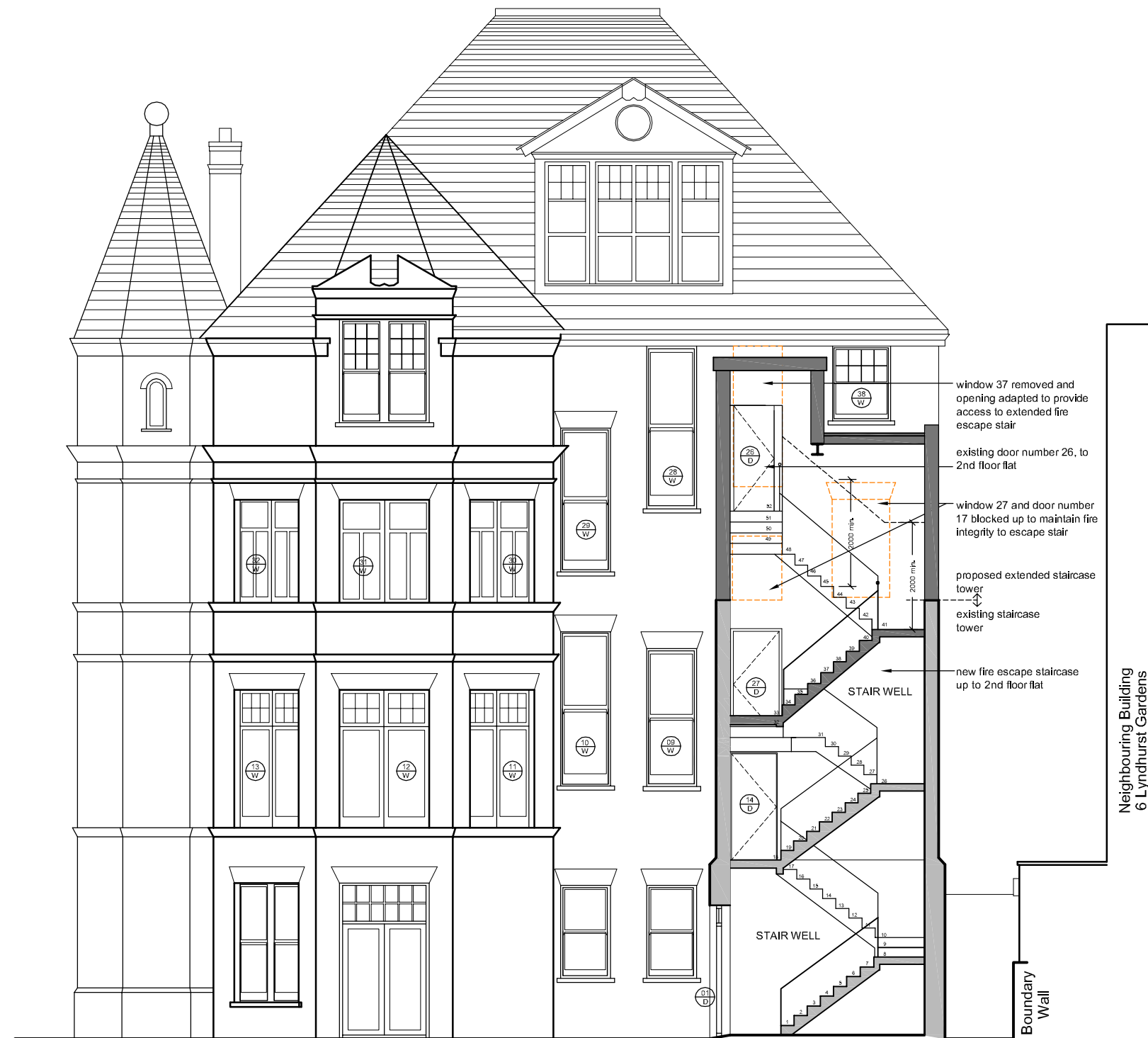
PROPOSED SECTION EE
