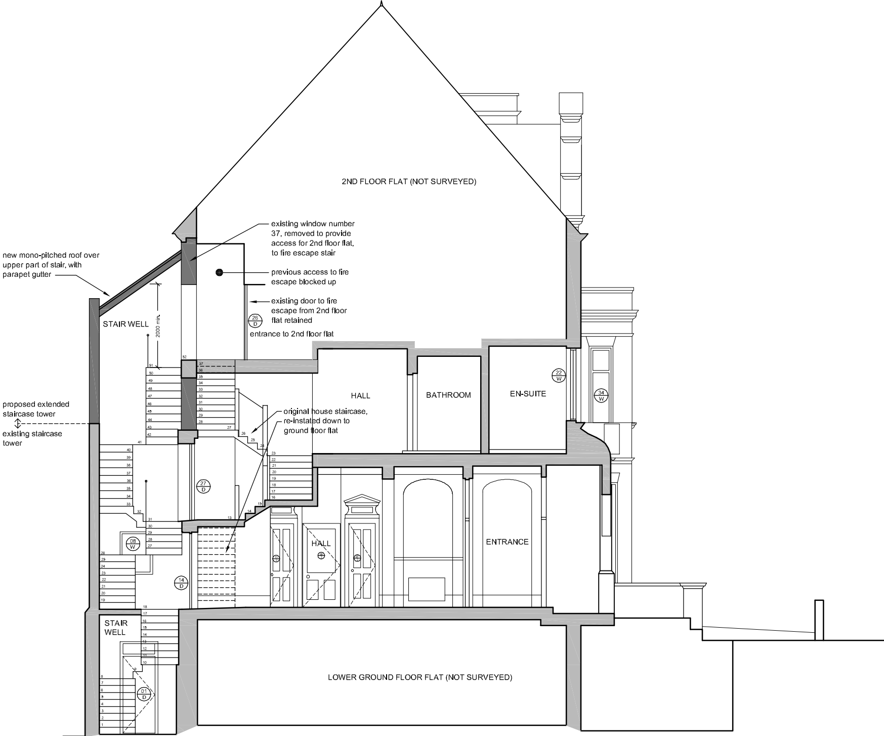
PROPOSED SECTION DD
