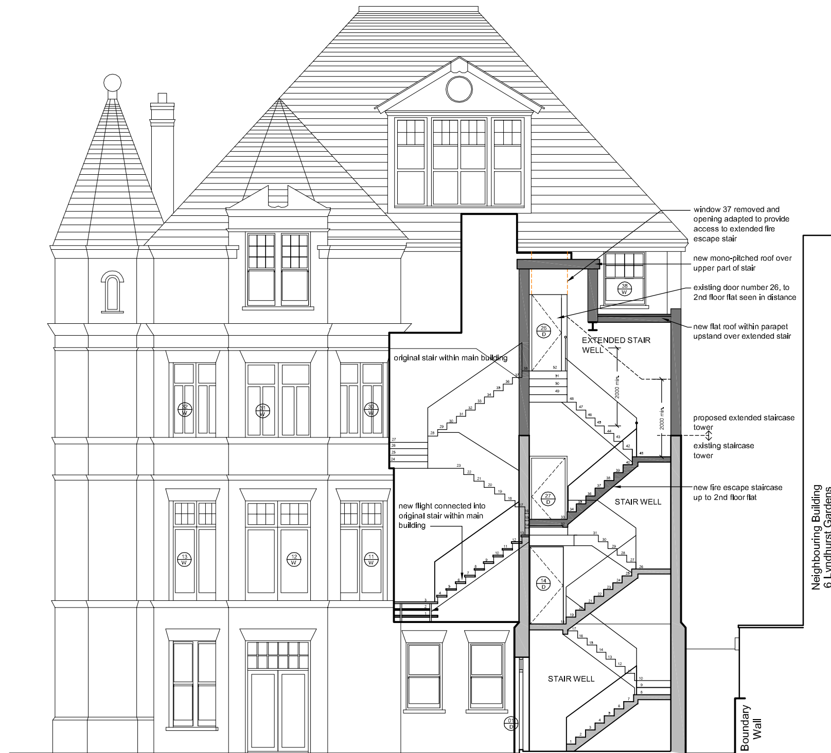
PROPOSED STAGGERED SECTION CC - THROUGH STAIRCASES
