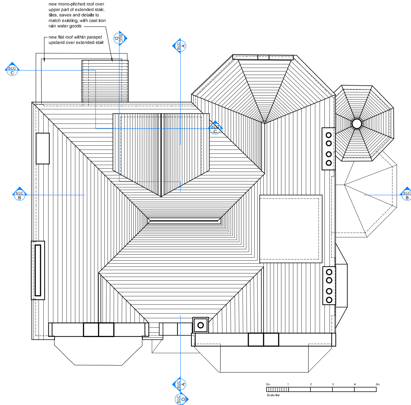
PROPOSED ROOF PLAN (note: assumed layout, roof not surveyed)
