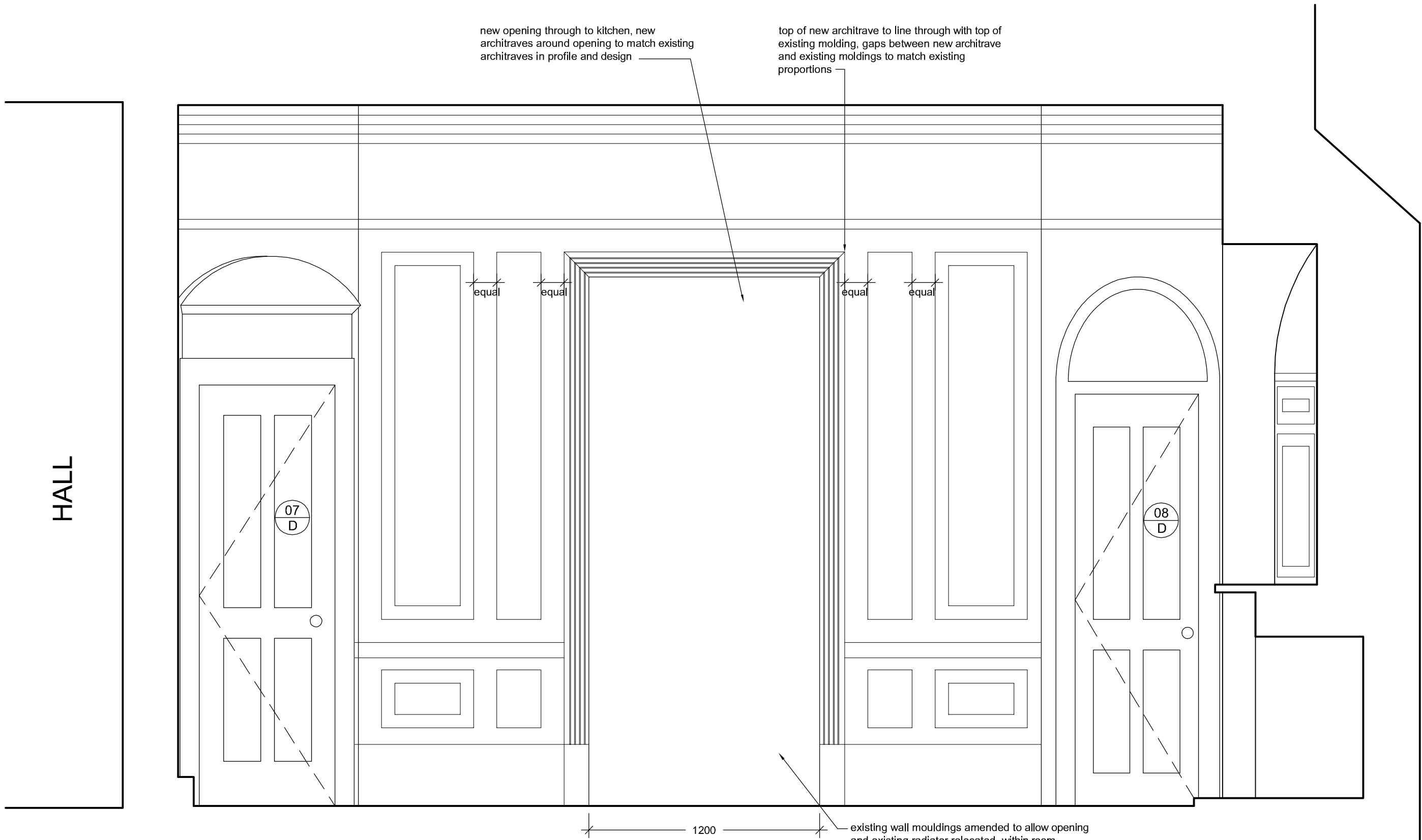
A1 PROPOSED INTERNAL ELEVATION - LIVING ROOM
