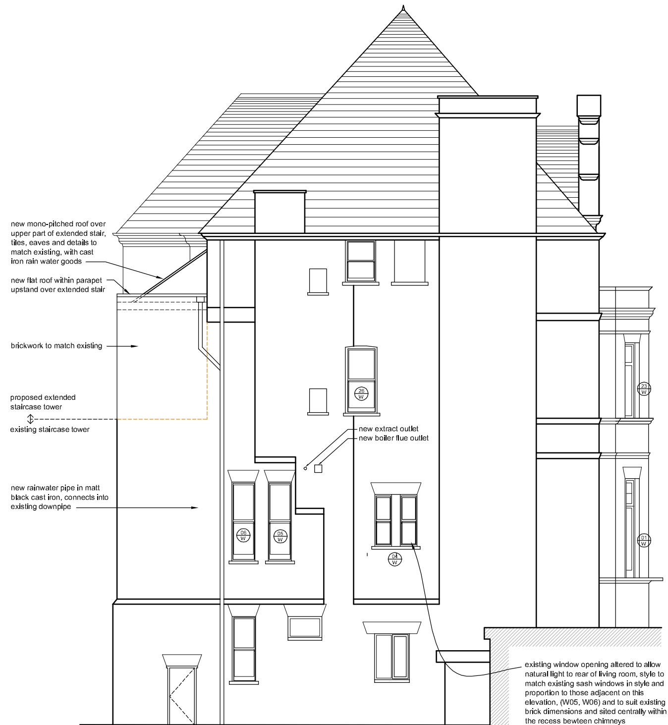
PROPOSED EAST ELEVATION - SIDE
