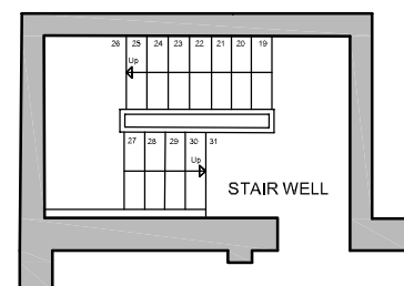
FIRST FLOOR EXISTING HALF LANDING FIRE ESCAPE STAIR
