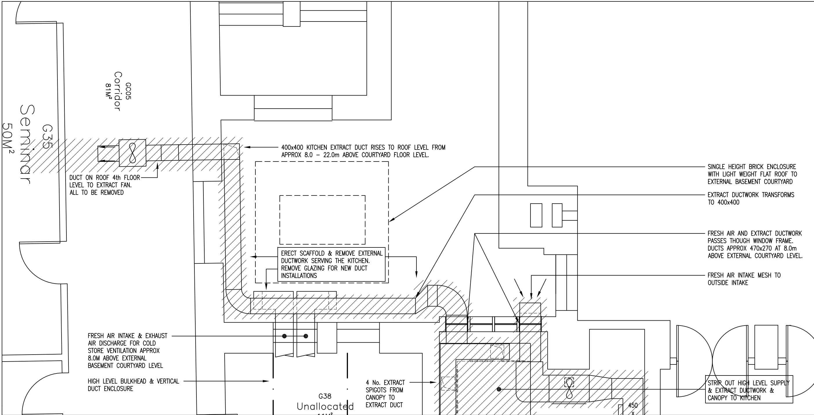
EXISTING ROOF AND COURTYARD PLAN LAYOUT
